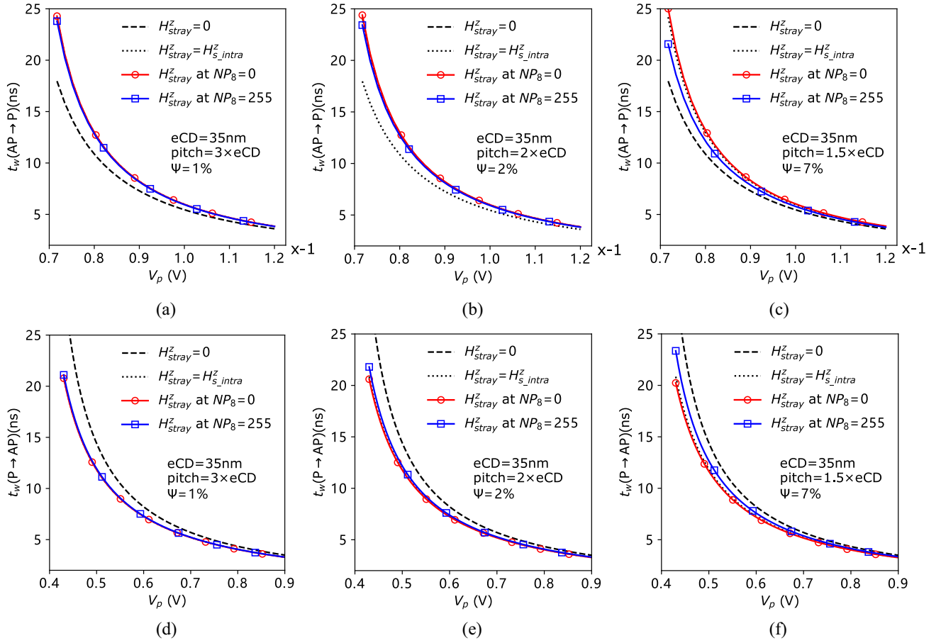
Fig. 5. Impact of internal stray fields on the voltage dependence of t_w with eCD = 35 nm at various pitches. (a) 3 \times eCD, AP \rightarrow P switching. (b) 2 \times eCD, AP \rightarrow P switching. (c) 1.5 \times eCD, AP \rightarrow P switching. (d) 3 \times eCD, P \rightarrow AP switching. (e) 2 \times eCD, P \rightarrow AP switching. (f) 1.5 \times eCD, P \rightarrow AP switching.
