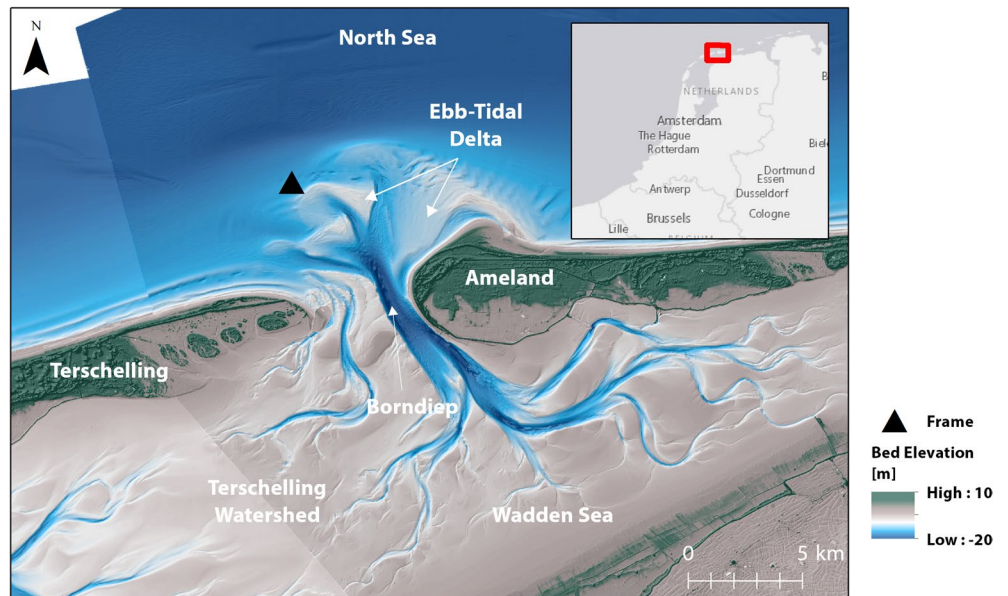
Figure 2. Overview of measurements during the September 2017 field measurement campaign at Ameland Inlet, including the frame (AZG-F4) bearing the instruments used in this study. Bathymetry source: Rijkswaterstaat Vaklodgingen. Elevation source: Actueel Hoogtebestand Nederland (AHN), Rijkswaterstaat. Basemap sources: Esri, HERE, Garmin, ©OpenStreetMap contributors, and the GIS user community.
