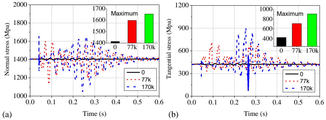
Figure 14. Wheel-rail contact stress comparison for different polygon samples: (a) normal stress; (b) tangential stress.
