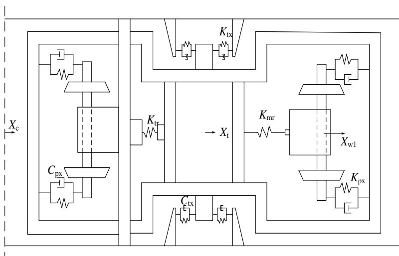
Figure 6. Side view of the locomotive-track model.
