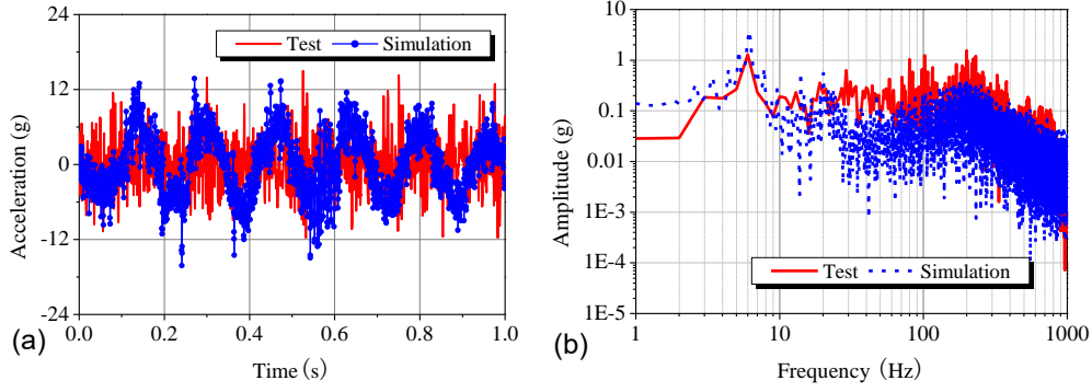
Figure 8. Comparisons of wheelset vertical acceleration in (a) time domain and (b) frequency domain.
