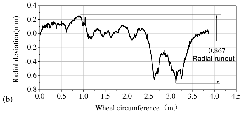
Figure 2. Wheel polygons of different mileage: (a) samples (b) definition of radial runout.
