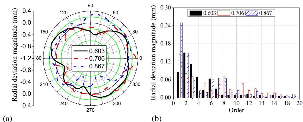
Figure 5. Serious wheel polygon wear: (a) wheel polygon; (b) order spectrum.
