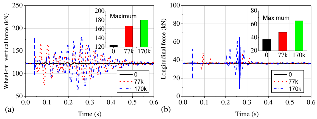
Figure 13. Wheel-rail dynamic force comparison for different polygon samples: (a) vertical forces; (b) longitudinal creep forces.
