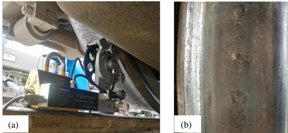
Figure 1. Field test of wheel polygon: (a) test scene; (b) tread shelling.
