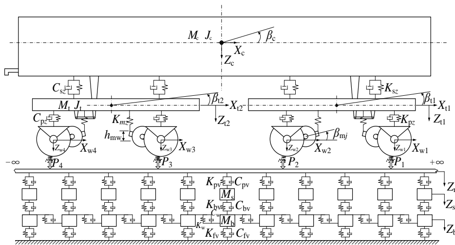
Figure 6. Side view of the locomotive-track model.
