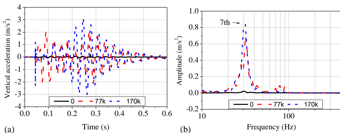
Figure 11. Vertical acceleration of wheelsets: (a) time response, (b) spectrum characteristic.
