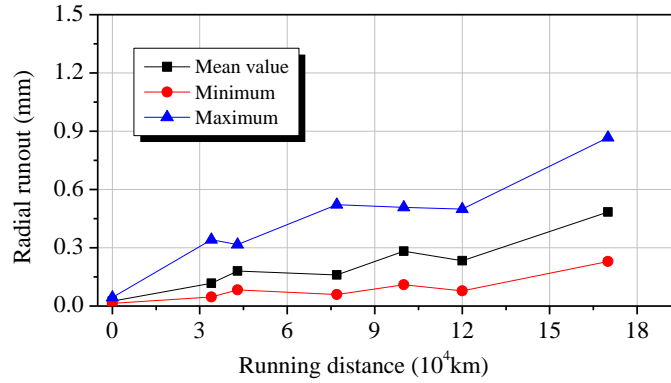
Figure 4. Statistical results of wheel radial runout.
