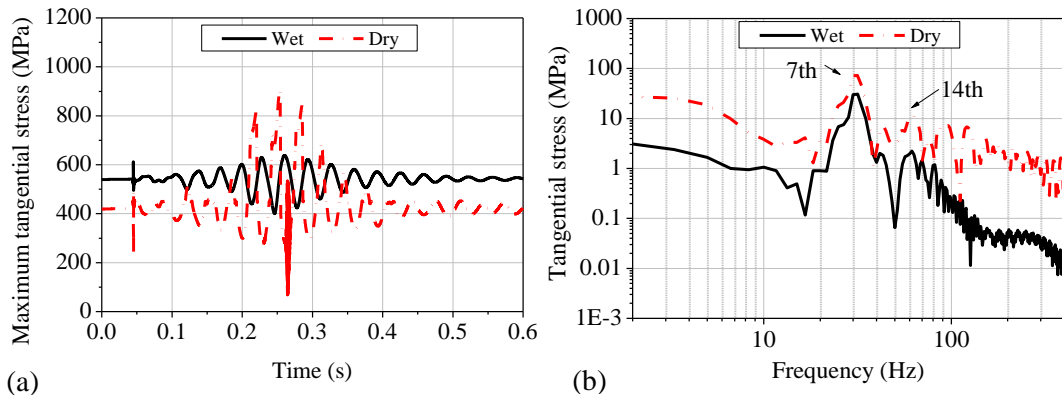
Figure 10. Wheel-rail tangential stress in dry and wet rail condition: (a) time response, (b) spectrum characteristic.
