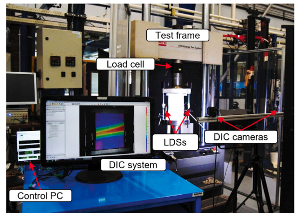
Fig. 7. Experimental test setup at Delft University of Technology showing the panel in a hydraulic universal testing machine together with the data acquisition used, such as the DIC and Laser displacement sensors (LDS).
