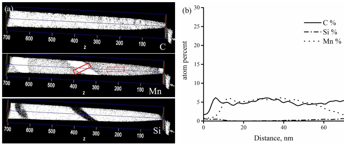
Fig. 4.12: The 3D element maps of APT needle taken in WEL, \sim 2 \mu\text{m} beneath the rail surface (a) and the composition quantifications of volumes in the empty rectangle in (b).
