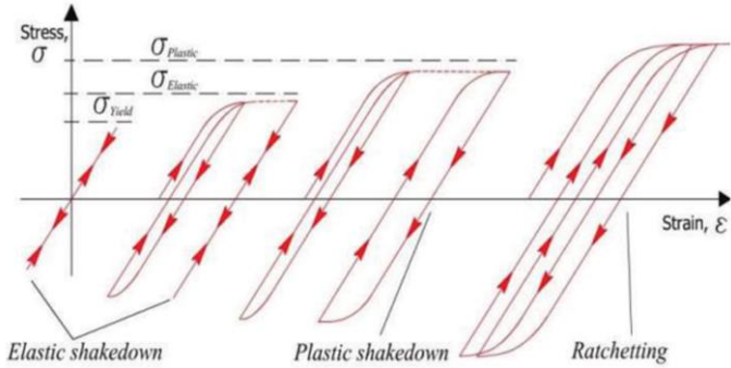
Fig. 2.3: The principal material response to the external cyclic loadings in rail steels [40]
