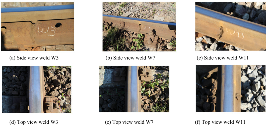
Fig. 4 Three different welds, W3, W7 and W11.
