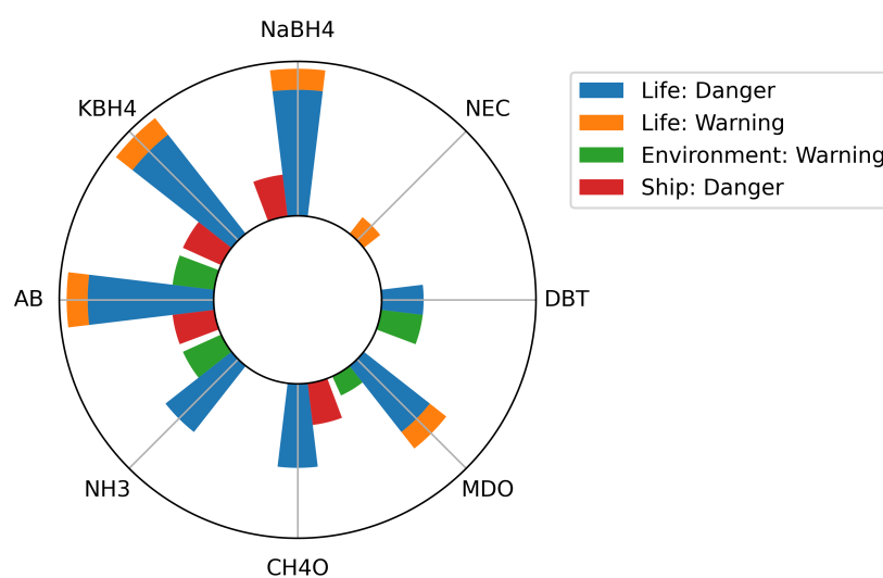
Figure 5. An overview of the alternative fuels and their hazards based on the three major focal points: life of on board (life), structural integrity of the ship (ship) and the aquatic environmental impact (environment), including the dangers and warnings stacked together. The bar height is based on the number of hazards per category, with D having more weight than W.
