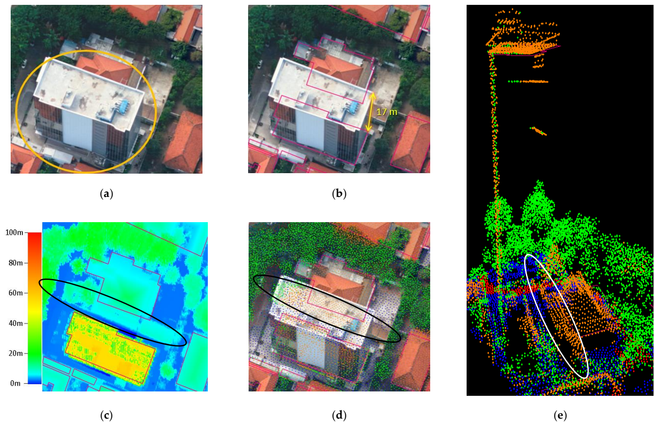
Figure 10. Relief displacement makes a high-rise building block an adjacent lower building and trees. (a) The leaning of a building (inside orange circle) on an orthophoto indicates relief displacement; (b) the building in the orthophoto has an offset of up to 17 m from the reference polygon (pink outlines); (c) the LiDAR DSM indicates a part of building that does not exist in the base map/reference (inside the black ellipse); (d) DGCNN can detect building points (orange) correctly, including the missing building part (inside the black ellipse); (e) 3D visualization of the classified building points including the missing building part (inside the white ellipse).
