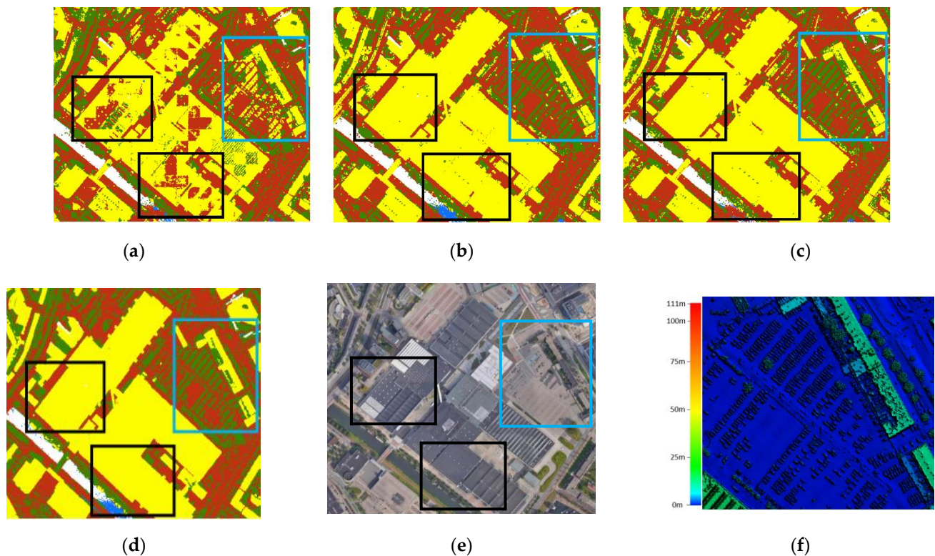
Figure 11. Visualization of point cloud classification results of a subtile in Area-2 (bare land in brown, buildings in yellow, water in blue, and “others” in green) in comparison with the ground truth. (a) Block size = 30 m, (b) Block size = 50 m, (c) Block size = 70 m, (d) Ground truth, (e) Satellite image ©GoogleMap2020, (f) DSM of the blue box shows that cars are categorized as “others”.
