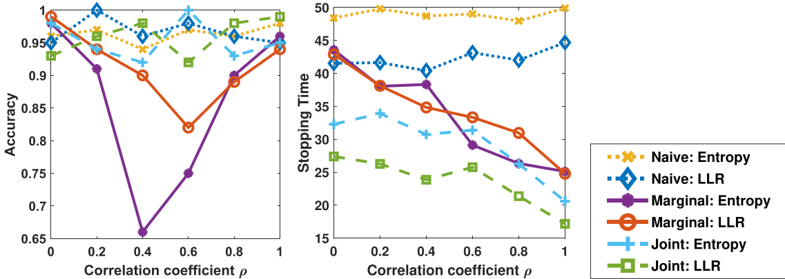
Fig. 4. Performances of different centralized deep actor-critic algorithms with varying \rho when \Upsilon_{\text{upper}} = 0.95 .
