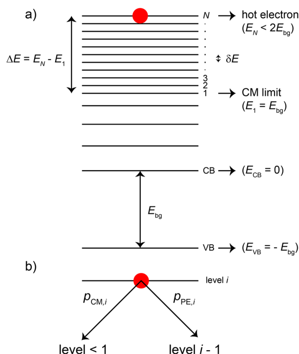
Figure 2. (a) Electronic structure for PbSe QDs. The CB energy is set to 0, such that the first energy level from which an electron can undergo CM has at least the band gap energy E_{\text{bg}} . This energy level is labeled 1. Above the minimal energy required for CM, we assume equidistant energy levels with N the highest level at which we initially create a hot electron. Since we only consider single CM events, this energy must be lower than twice the band gap energy. (b) Possible scenarios of phonon emission or CM from an energy level i .
