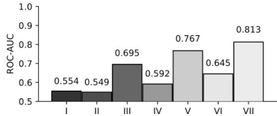
100-taxa Vertebrate PhyloP
