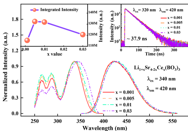
Figure 4. Highest height-normalized emission ( \lambda_{\text{ex}} = 340 nm) and excitation ( \lambda_{\text{em}} = 420 nm) spectra of Li 1+x Sr 4–2x Ce x (BO 3 ) 3 (x = 0.001, 0.005, 0.01, or 0.03) at RT. The insets show the integrated intensity of emission spectra and the fluorescence decay curves ( \lambda_{\text{ex}} = 320 nm, and \lambda_{\text{em}} = 420 nm) of Li 1+x Sr 4–2x Ce x (BO 3 ) 3 .
