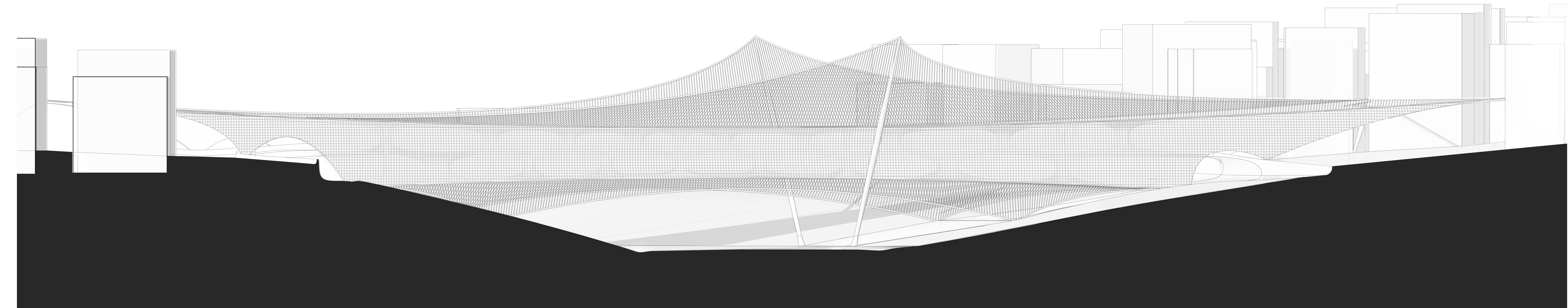
East Elevation 1:200
