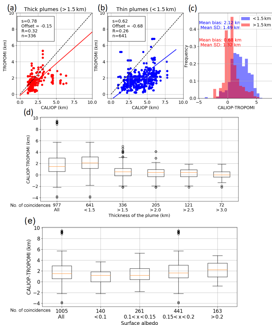
Figure 4. CALIOP–TROPOMI comparison for (a) geometrically thick plumes (> 1.5 km) and (b) geometrically thin plumes (< 1.5 km), together with the statistics of the line of best fit (correlation coefficient, R , slope, s , and number of observations, n ). The plume thickness is determined by the CALIOP top and base plume height. Panel (c) shows the histogram for the differences in plume height (CALIOP – TROPOMI) for thick (red) and thin (blue) plumes. Panel (d) shows the statistics for different plume thickness filters and (e) for different ranges of surface albedo.
