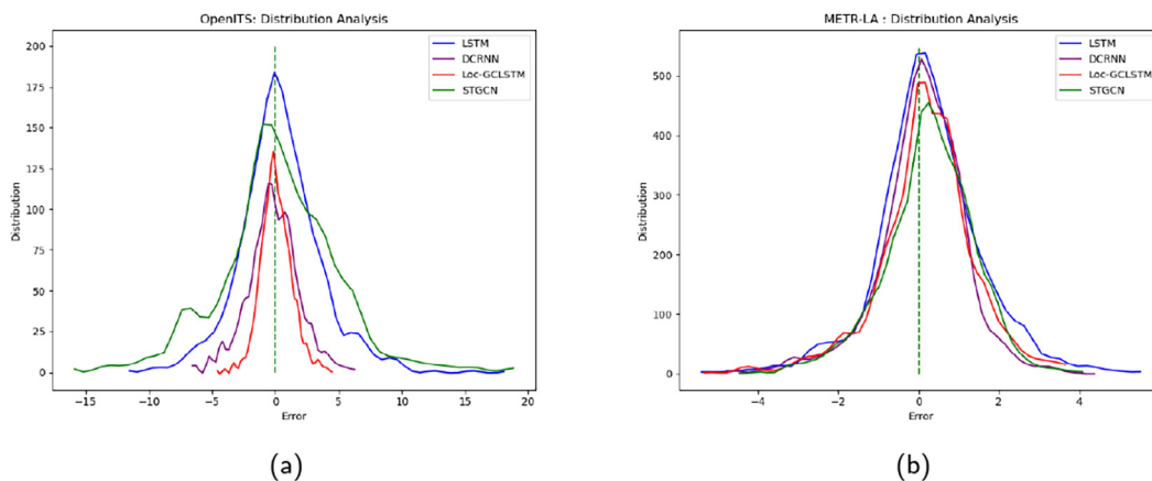
Fig. 10. Comparison between the distribution of prediction errors on (a) OpenITS dataset; (b) METR-LA dataset.
