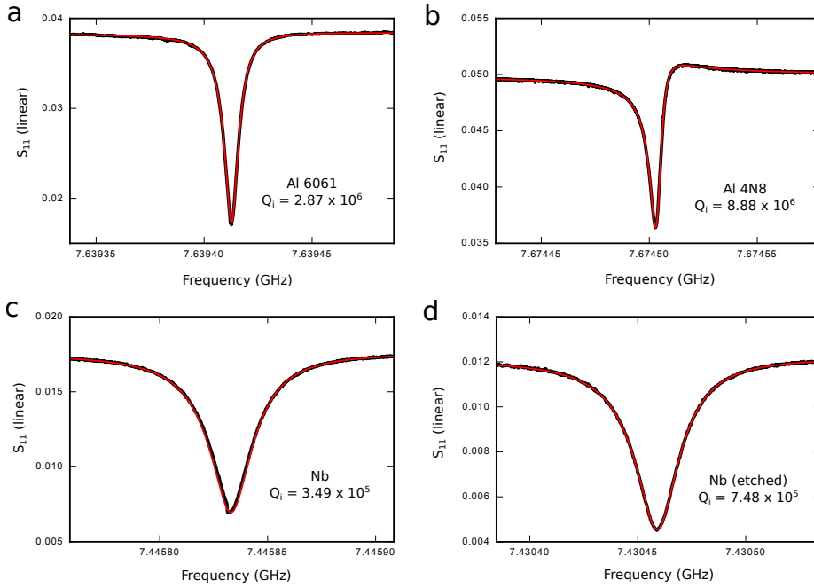
Figure 3.6: Reflection coefficients measurements for four different 3D cavities, black line is the raw data and the red line is a lorentzian fit. (a) 6061 aluminium alloy, (b) 4N8 (99.998%) purity aluminium, (c) unetched niobium, (d) etched niobium. The aluminium cavities were measured at 16 mK, and the niobium cavities were measured at 4.2 K. A summary of the fitted data can be found in table 3.1
