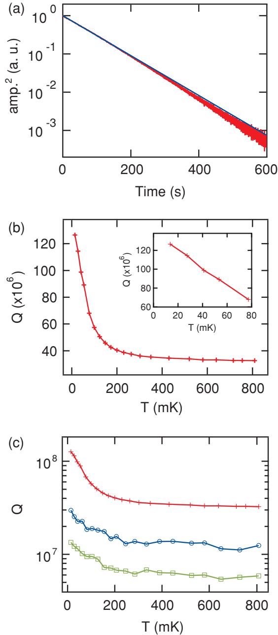
Figure 4.3: (a). Time trace of the mechanical amplitude during ringdown for Device I at 14 mK. From a fit to exponential decay, we extract the mechanical quality factor. Red: data; blue: fit. The deviation from a straight line may indicate some weak negative nonlinear damping. (b). Extracted quality factor Q of the membrane resonator as a function of cryostat temperature for Device I (1,1) mode. Inset: zoom-in for T < 80 mK. The highest value is Q = 1.27 \times 10^8 for Device I at 14 mK. (c). Extracted quality factor for both samples. Red: Device I (1,1) mode; blue: Device II (1,1) mode; green: Device II AS mode. Q decreases with increasing temperature for 14 \text{ mK} < T < 200 \text{ mK} , leveling out between 200 mK and 800 mK.
