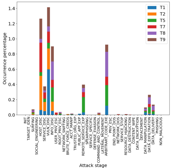
Fig. 2. The distribution of alerts per attack stage for the CPTC-2018 teams. Scanning-alerts are significantly more frequent than exploitation-alerts.
