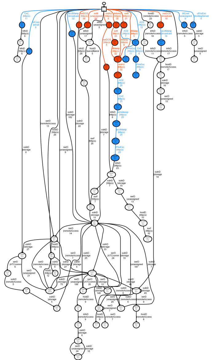
Fig. 6. The S-PDFA model for CPTC-2018. The states are colored according to the severity of the incoming symbol's attack stage: red is high, blue is medium, white is low.
