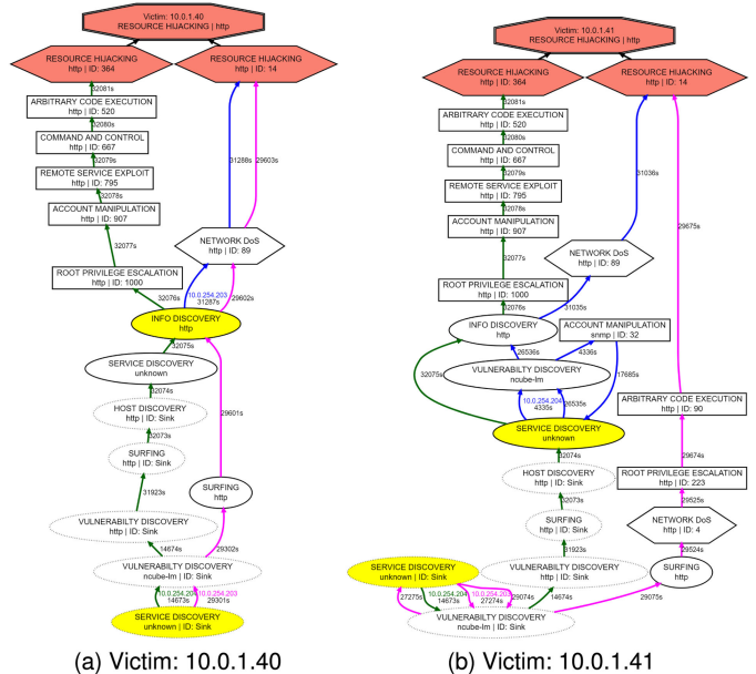
Fig. 11. Similar attacks targeting multiple victim hosts result in overlapping attack graphs.
