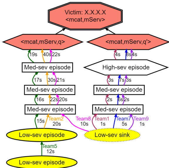
Fig. 7. An alert-driven attack graph: Vertices: Labels show \langle attack\ stage, targeted\ service, state\ identifier \rangle . Low-severity episodes are oval, medium-severity are boxes, high-severity are hexagons. The first episode in a path is yellow, the objective is black. Sinks are dotted. Edges: Labels show seconds since the first alert. Colors show team affiliation: T1 (Maroon), T2 (Orange), T5 (Green), T7 (black), T8 (Magenta), T9 (Purple).
