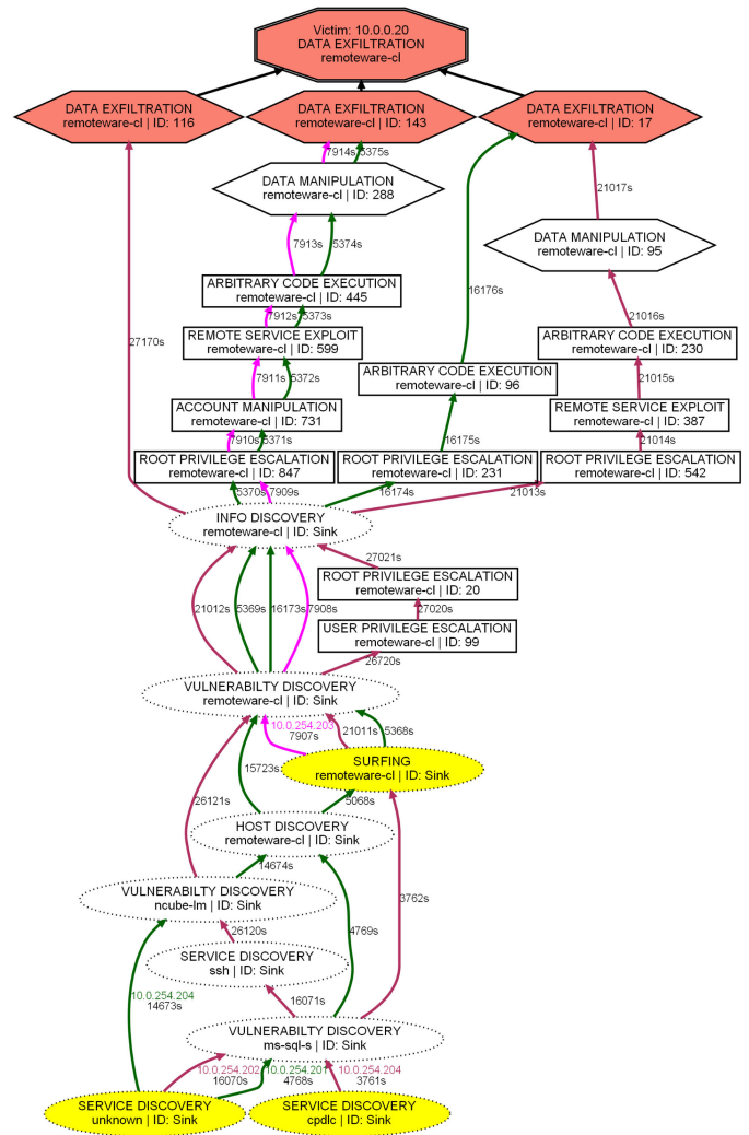
Fig. 8. Attack graph of data exfiltration over remoteware-cl. Three attacker teams successfully exploit it. Teams 1 and 5 exploit it twice, and each subsequent attempt is shorter than the first. The S-PDFA identifies three ways of exploiting the objective based on the actions that lead up to it.
