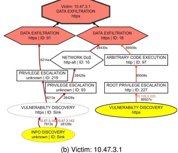
Fig. 14. Highly similar attack graphs of two victims from CCDC-2018. The graphs are identical, except for an additional attack attempt by a new attacker in the second graph.
