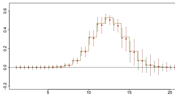
(a) Low noise (10%); small sample size ( N = 50 )
