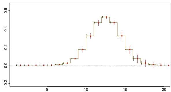
(b) Low noise (10%); large sample size ( N = 500 )
