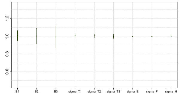
(d) High noise (50%); large sample size ( N = 500 )
