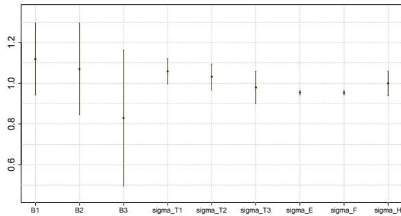
(c) High noise (50%); small sample size ( N = 50 )
