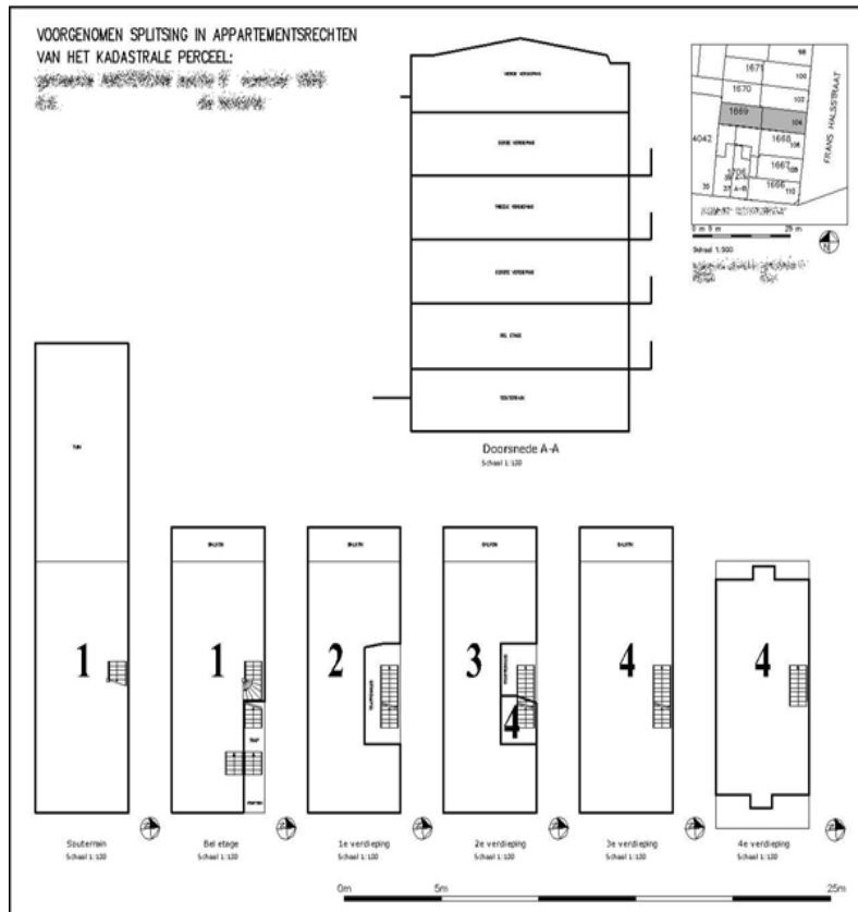
Figure 2.6.1. Example of a drawing (“splittingssteking”) providing an overview of the apartment complex. The boundaries of the private parts are indicated by a thick black line.
