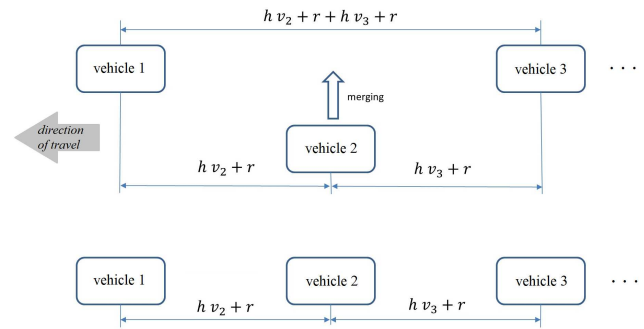
Fig. 3: Spacing policy during and after merging (only vehicles 1, 2, 3 are shown). The spacing is calculated with respect to the vehicle center of mass for simplicity.
