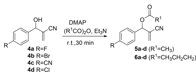
Scheme 2. Synthesis of MBH esters.
