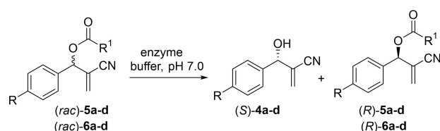
Scheme 3. Enzymatic kinetic resolution of 5 and 6.
