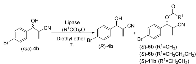
Scheme 4. EKR by transesterification reaction of 4b .
