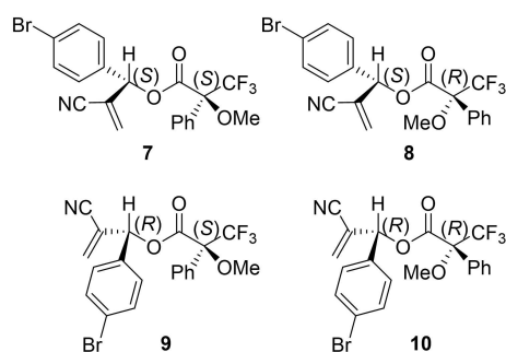
Figure 1. Mosher's ester derivatives of 4b .
