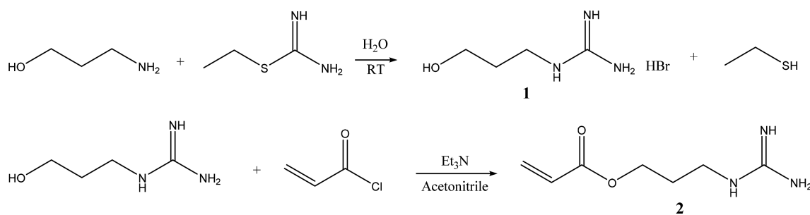
Scheme 1. Reaction Scheme for the Two-Step Synthesis of (1) Guanidinium Propanol and (2) the Guanidinium Acrylate Monomer
