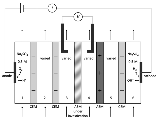
Figure 1. Scheme of the setup used to perform electrochemical impedance spectroscopy and electro dialysis experiments. CEM and AEM denote cation- and anion-exchange, standard-grade membranes, respectively. The membrane under investigation was positioned between compartments 3 and 4. The current was supplied from two counter electrodes positioned in compartment 1 (anode) and compartment 6 (cathode).
