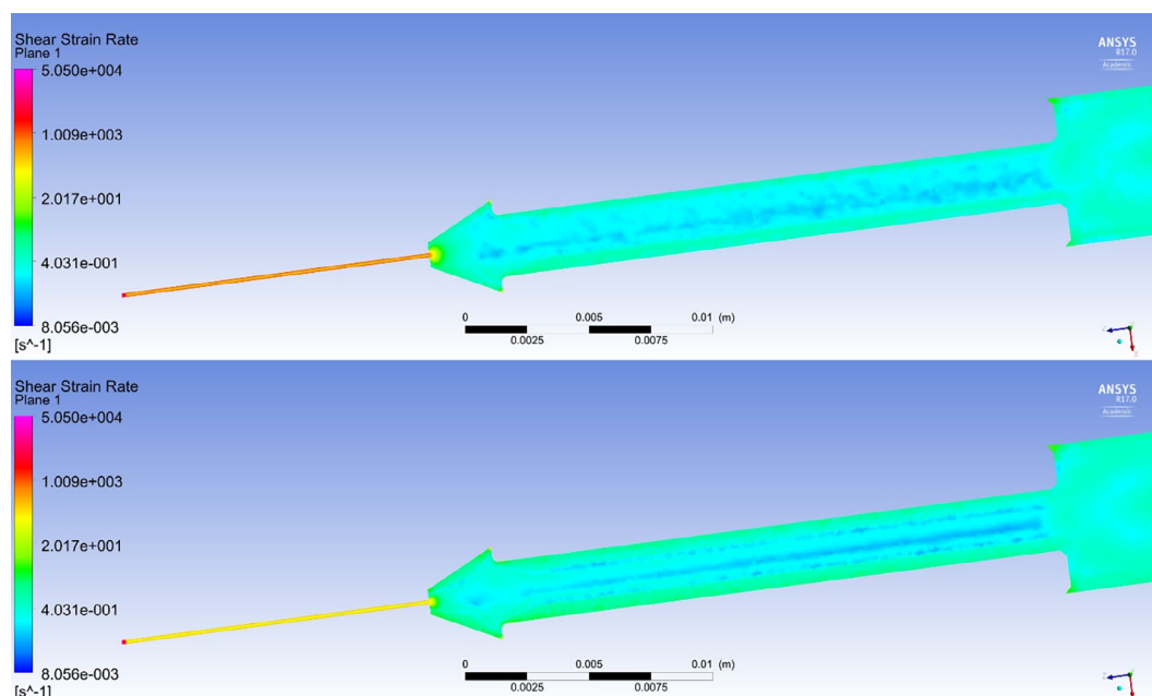
Figure 7. Simulated shear rate distribution for \eta = 10 Pa s and rotation rates 10,000 rpm (top) and 5,000 rpm (bottom). The shear rate magnitude increases due to the higher centrifugal forces produced by the faster rotation. The highest shear rates occur in the region where the polymer exits the die. [Color figure can be viewed at wileyonlinelibrary.com ]
