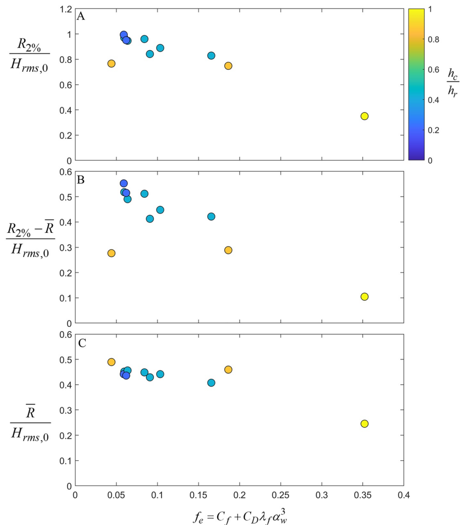
Figure 13. The 2% exceedance wave runup (a), 2% exceedance swash, and (c) wave setup at the shoreline with each normalized by deep water rms wave height versus wave energy dissipation factor f_e calculated following Lowe et al. (2007) using canopy geometry. In the calculation, the incident peak wave period is used and a rms velocity of 0.1 m/s is assumed based on observations near the reef crest. The colormap gives the relative submergence of roughness elements on the reef flat for still water level conditions. The forcing conditions, fore-reef slope, reef flat length, and beach slope from Run 2 were used.
