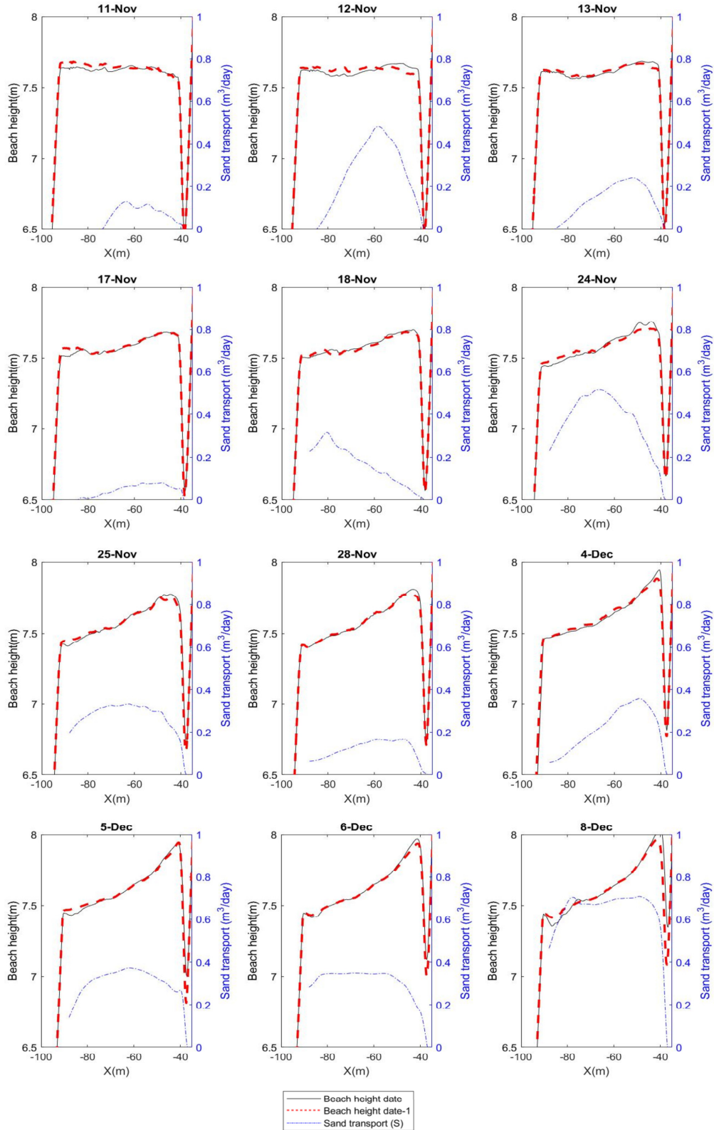
Figure 9: Estimated cross-shore sand transport ( Q_s ) based on formula 2 for days that sand transport could be identified (blue dashed line). Next the plots show the beach profile for the date specified in the title (black line) and the beach profile of the day before (dashed red line).
