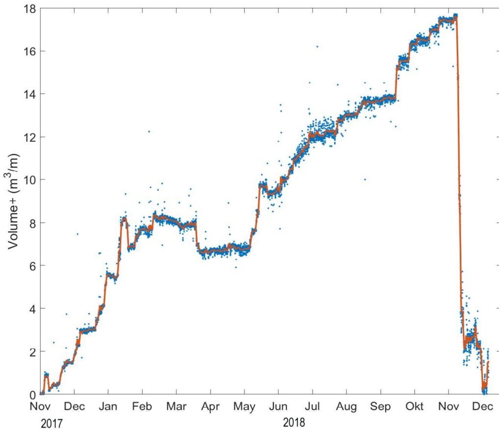
Figure 7: Averaged sand volumes (along the alongshore axis) in the berm above the first reference scan (consisting of a flattened beach) in \text{m}^3/\text{m} over the measuring period. The scatter plot shows individual volumes with the red line showing a time averaged trend (averaging period 24 hours). Points around July 2018 show a large scatter due to problems with the time dependent corrections.
