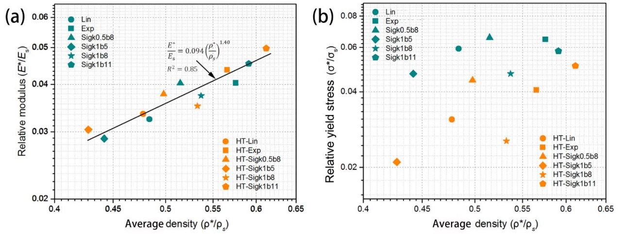
Fig. 14 (a) Relative Young's modulus and (b) relative yield strength in relation to the overall density of the FGSSs.
