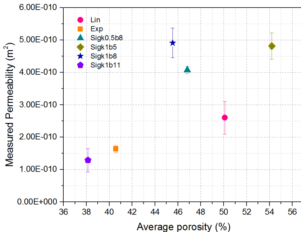
Fig. 10 Permeability of functionally graded scaffolds.
