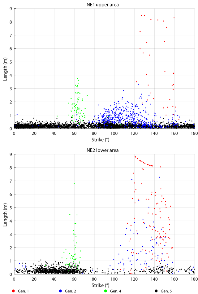
Figure 17. Plots of strike direction ( ^{\circ} ) on the x axis and length (m) on the y axis for every fracture mapped in the domains in the NE and color coded by generation.
