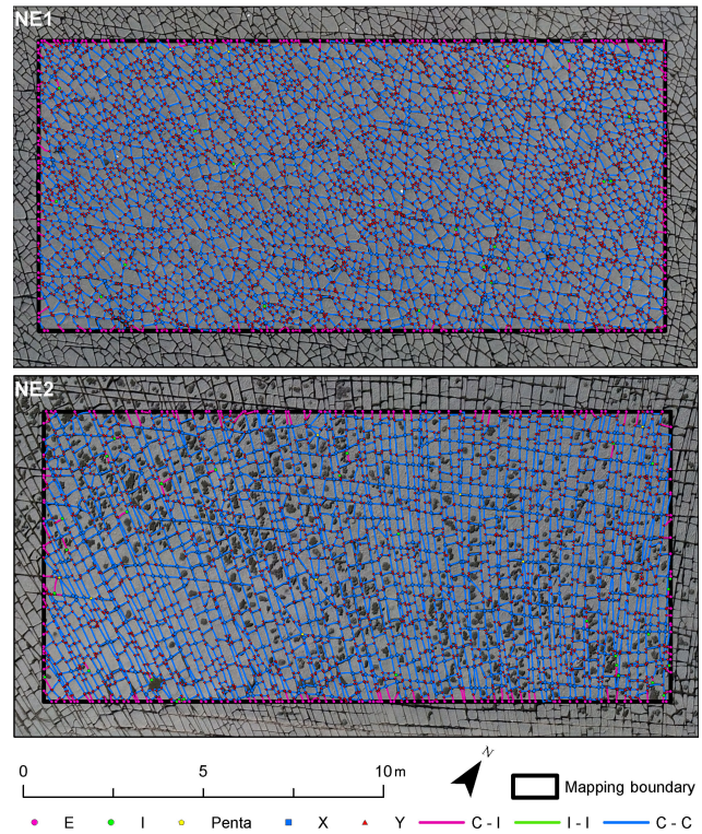
Figure 11. NE fracture networks, automatically traced and plotted as branches and nodes.
