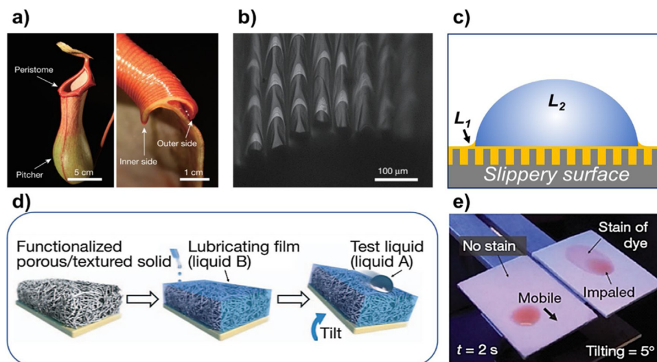
Fig. 5 – An emerging type of self-cleaning surfaces inspired by Nepenthes pitcher. a, b) Optical images of Nepenthes Alata and Microstructure surface from the Nepenthes Alata . The microchannel structures with arch-shaped cavities effectively guide the liquid flowing (Chen et al., 2016). Copyright 2016, Macmillan Publishers Limited. c) The mechanism under the slippery surface. The surface energy is controlled by the mediated liquid ( L_1 ) irrespective of the solid surface underneath, as there is no direct contact between the test liquid and the solid surface. d) The prototype of slippery liquid-infused porous surface (SLIPS) inspired by Nepenthes pitcher. e) The self-cleaning properties of SLIPS (left side in the image) compared to superhydrophobic surfaces (right side in the image). The test liquid is dyed Pentane and the test clearly shows the Pentane drop can be mobile on the SLIPS without a trace (Wong et al., 2011). Copyright 2011, Macmillan Publishers Limited.
