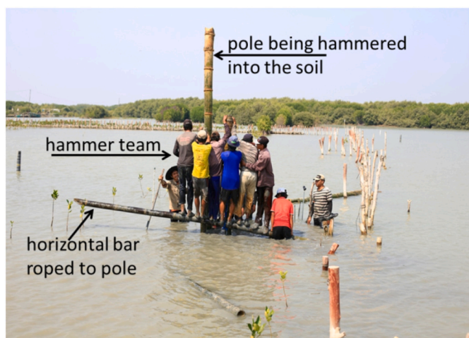
Fig. 32. Hammer team at work to place bamboo pole, Bogorame, Demak, Indonesia.
