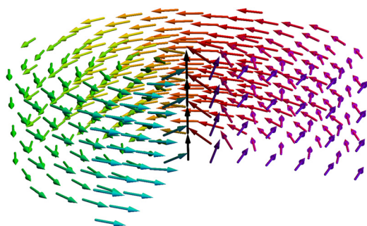
Fig. 1 Cylindrical magnetic dot in the vortex state (not to scale), arrows represent spin momenta directions of individual spins in the cubic lattice. The color of the spins corresponds to the direction of the planar component of the spin, spins on the axis of the particle point out of plane and form the core of the magnetic vortex.
