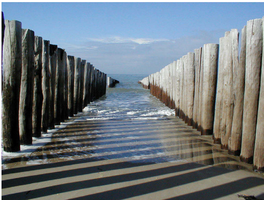
Figure 10.14: A row of piles serving as a groyne at the Zeeland coast in March 2004. This is only one of many types of groynes. Photo by Ad Reniers (see Credits on page 575).
