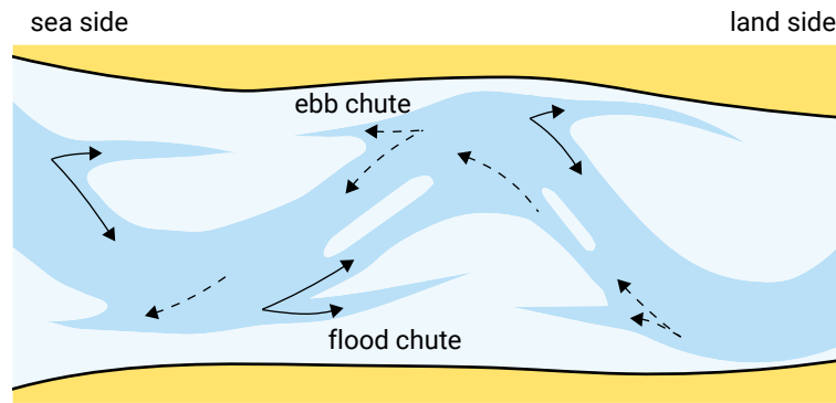
Figure 9.24: Meandering tidal channel with ebb and flood chutes (in Dutch: ebscharen and vloed-scharen ).
