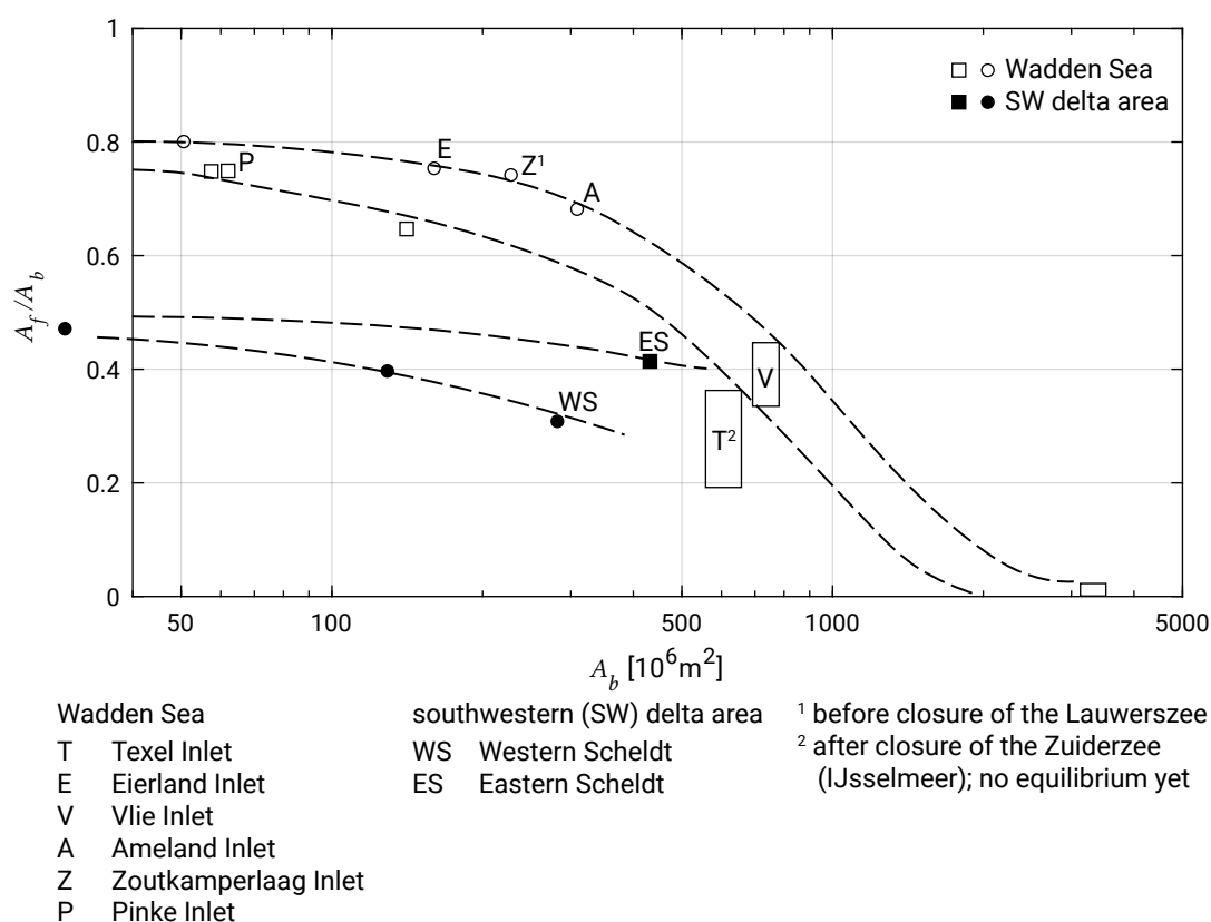
Figure 9.26: Relative area of the intertidal zones in the Dutch Wadden Sea (upper two lines) and the delta area in the southern Netherlands (lower two lines). Some of the inlet systems are indicated by letters.
