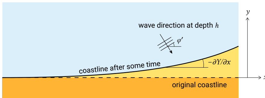
Figure 8.9: Shoreline position Y in original position and after some time. In this figure \varphi' is the original angle of wave incidence. After the change in shoreline orientation, this angle has been reduced with \partial Y / \partial x .
