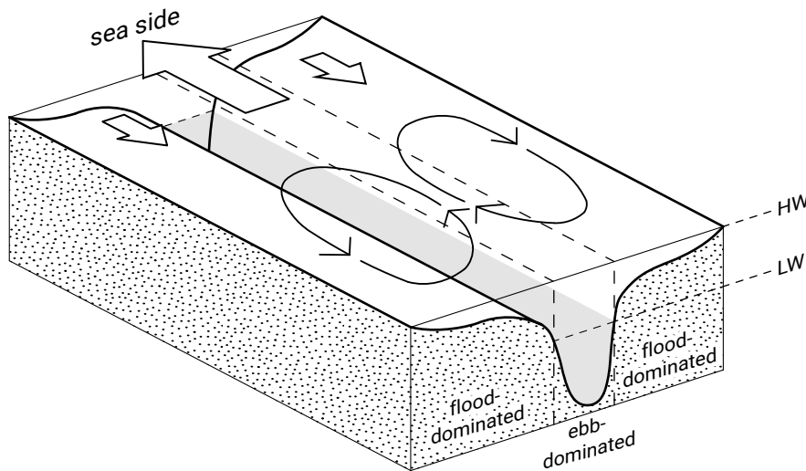
Figure 5.75: Bathymetry-induced circulation.
