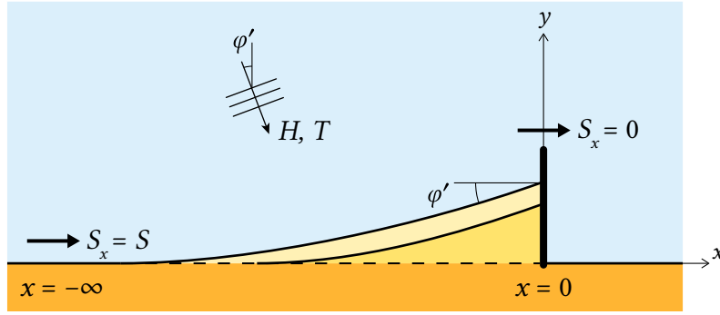
Figure 8.11: Accretion of the shore near a breakwater at different times. The wave conditions given in the sketch refer to the conditions at the assumed horizontal part in the coastal area.
