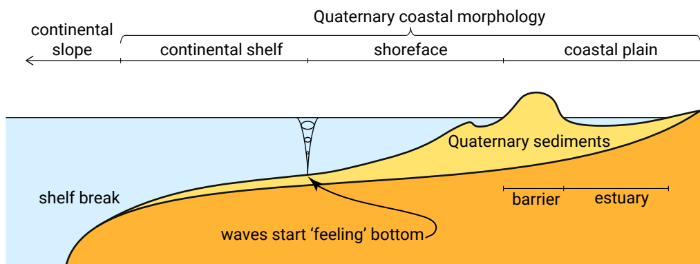
Figure 1.15: Spatial boundaries of the coastal zone. The Quaternary coastal morphology reaches up to the shelf break. The transition between the shelf and the shoreface is located where waves propagating towards the shore start feeling the bottom.
