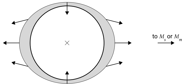
Figure 3.18: The direction and relative magnitudes of the differential gravitational pull at different locations on the earth's surface. At each location, it is given by the vector subtraction of a_{s \text{ or } m, \text{local}} and the part a_{s \text{ or } m} that provides the centripetal acceleration. The depicted tidal bulges result from the tangential components of the differential pull (see Fig. 3.19).
