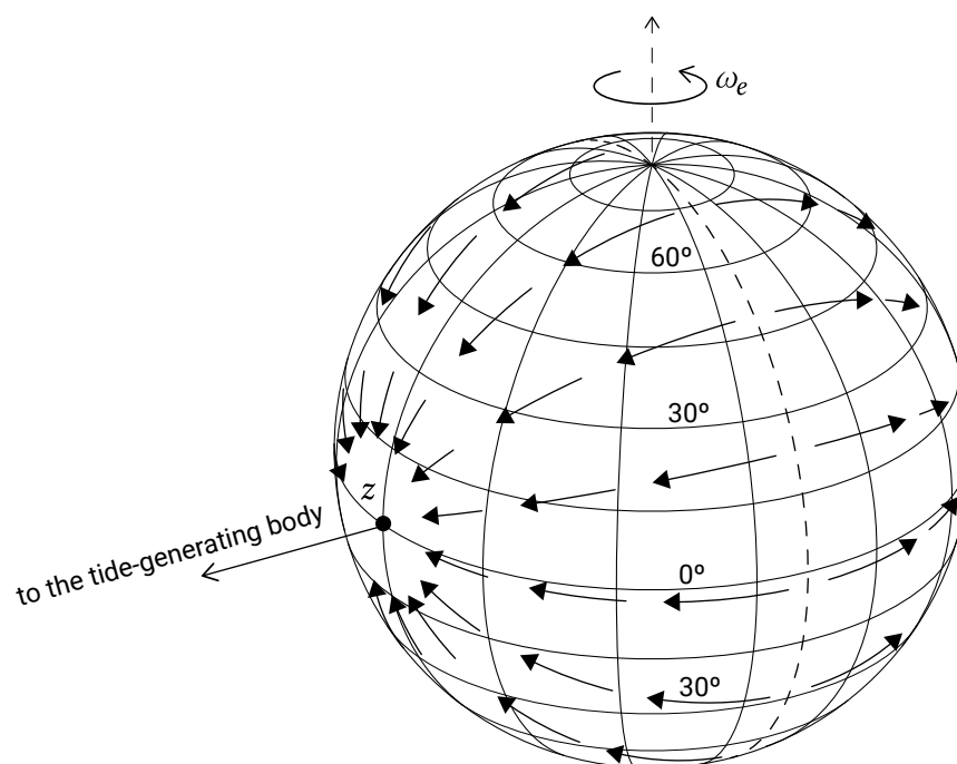
Figure 3.19: The horizontal component of the tidal force on the earth when the tide-generating body (the sun or the moon) is above the equator at z .
