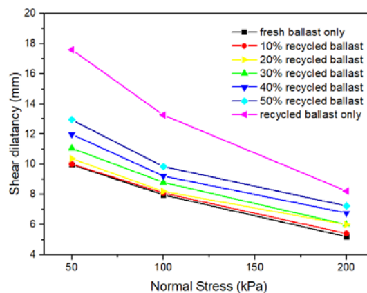
Fig.6 Shear dilatancy
