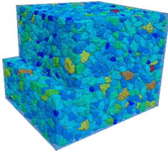
Fig. 11 The DEM numerical model of ballast direct shear test
