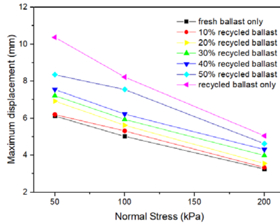
Fig.15 Maximum displacement
