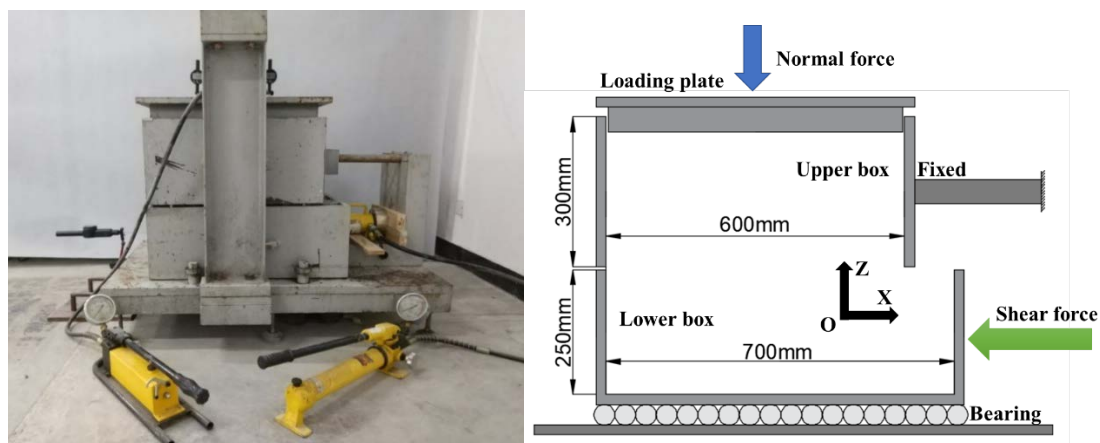
Fig.3 Large-scale direct shear apparatus
