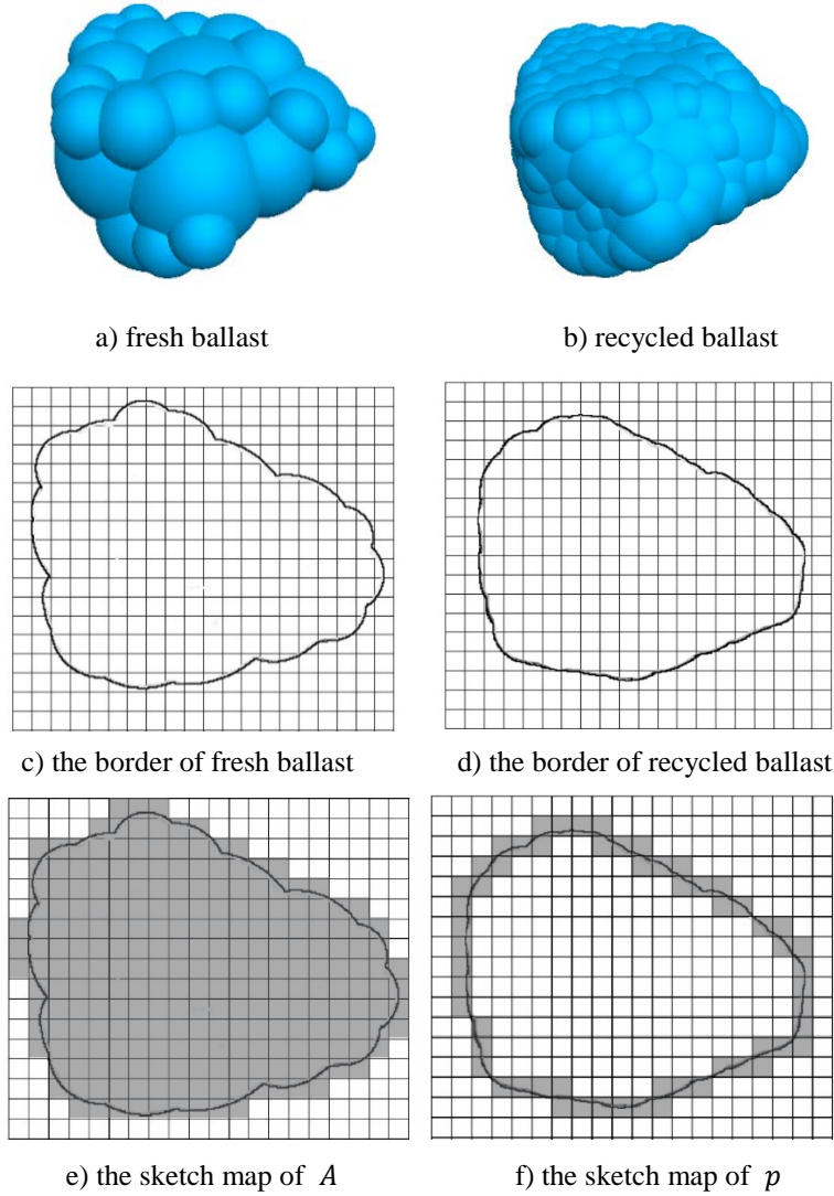
Fig. 10 Ballast particle models in DEM simulations
