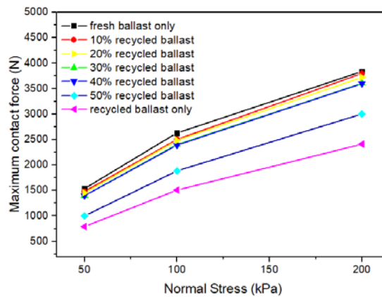
Fig.14 Maximum contact force
