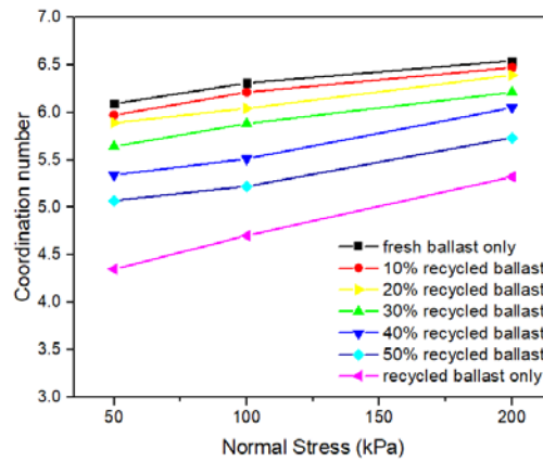
Fig.13 Average coordination number
