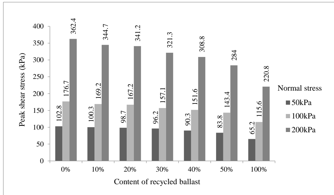
Fig. 4 Shear strength under different normal stresses
