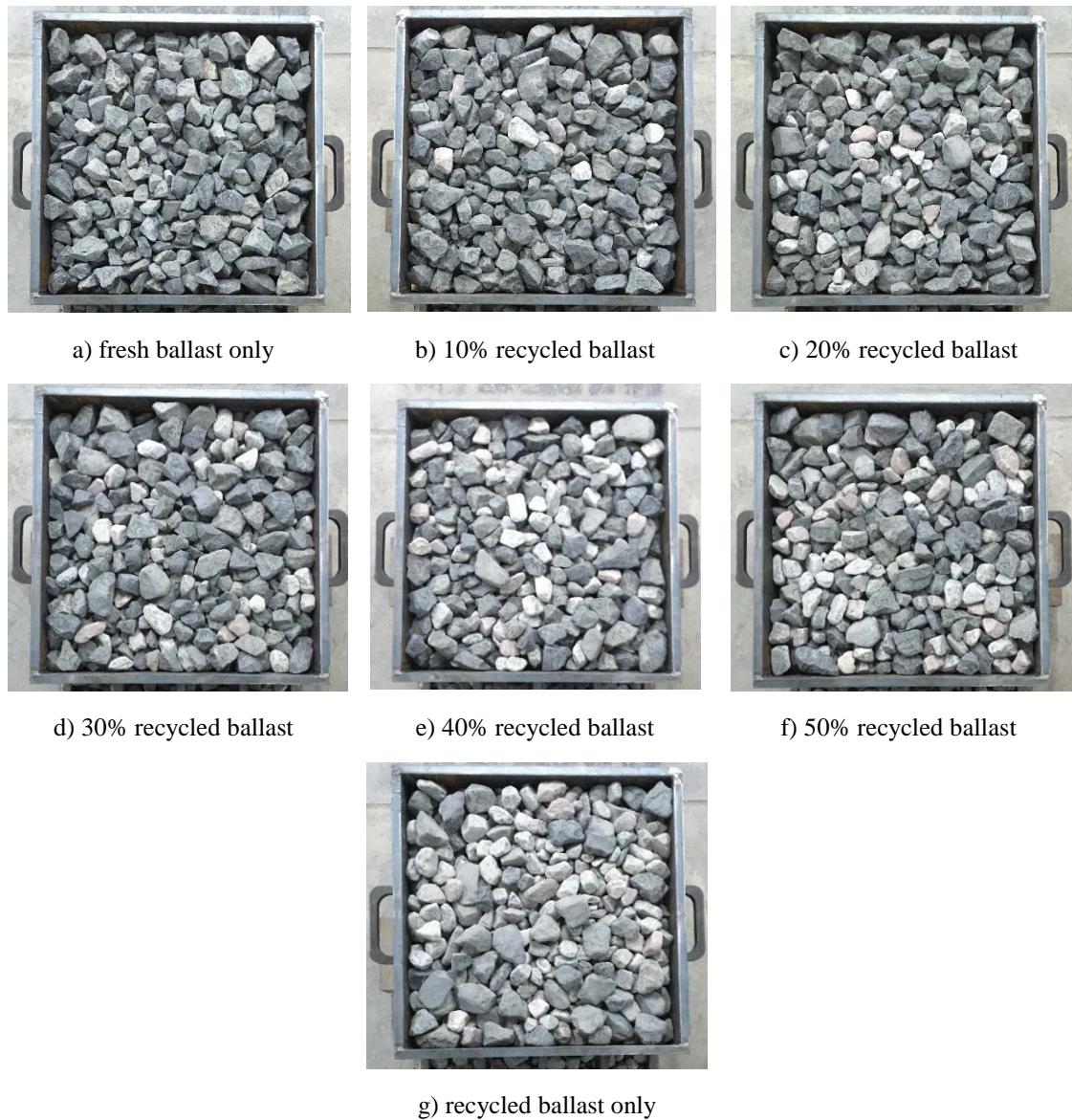
Fig. 2 7 specimens depending on the mixing ratio of recycled ballast
