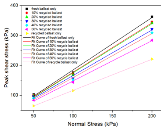
Fig.5 Linear fitting between normal stress and shear stress
