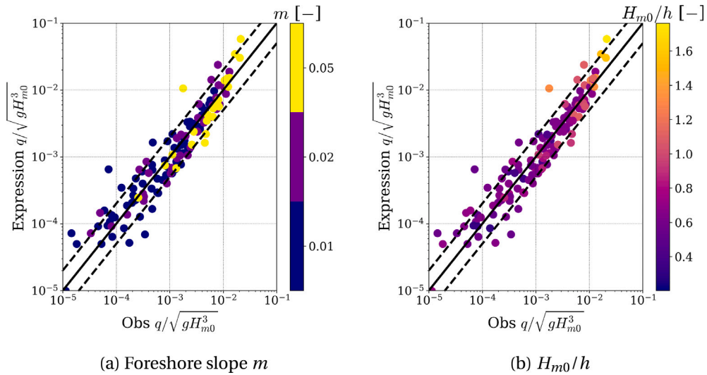
Fig. 12. Scatter plot of non-dimensional mean overtopping discharges between the observation (x-axis) and the model (y-axis). Next to the scatter, the 1:1 line and factor two lines ( \times 2 , \times 0.5 ) are shown in black. The left panel shows the scatter with the colours indicating the foreshore slope and the right panel shows the scatter with the colours indicating the relative water depth ( H_{m0}/h ).
