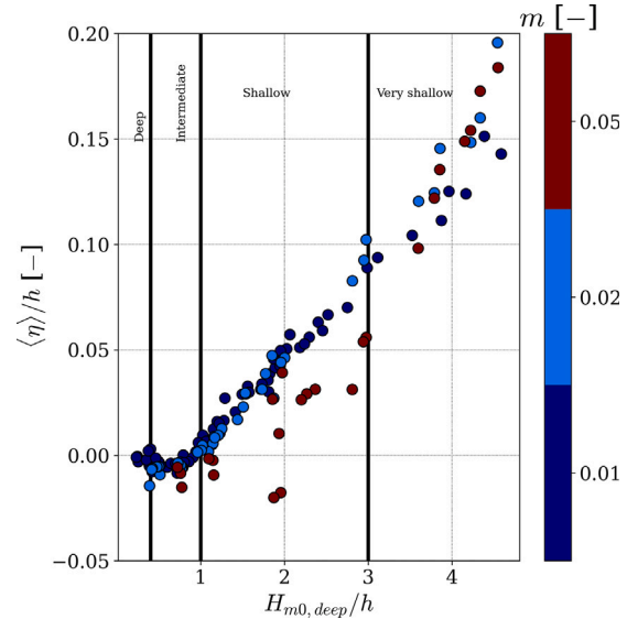
Fig. 6. Non-dimensional wave setup as a function of the relative water depth. The foreshore slope is shown with the marker colour. The results are obtained from Wave gauge WHM07 (in front of the structure). The black vertical lines show the limits of the regions: deep, intermediate, shallow and very shallow.
