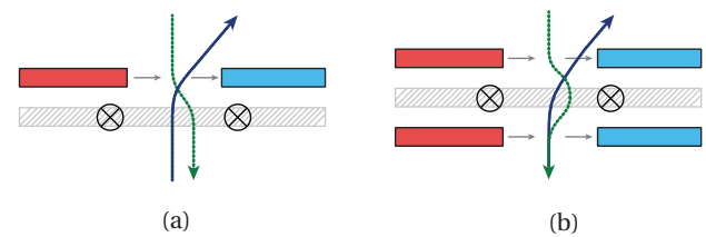
FIG. 2. (a) Schematic beam path through two consecutive dipole fields (one electric, one magnetic) and (b) the schematic beam path through three consecutive dipole fields (two electric, one magnetic). The electric field is distributed equally among the top and bottom layer and balances the deflection through the middle magnetic field. Notice that the role of magnetic and electric fields can be interchanged.
