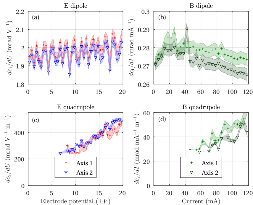
FIG. 12. (a) Electric and (b) magnetic dipole magnitudes, and quadrupole (c) electric and (d) magnetic magnitudes obtained for both axes in the E-B-E configuration. Results obtained at 2 keV beam energy.
