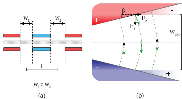
FIG. 6. (a) Gap width mismatch as seen from the side between both axes results in a net deflection error that is proportional to the deflection angle and variation in gap width. (b) A wedge geometry as seen from above leads to a quadrupole contribution to the deflection field, that would ordinarily be absent when \beta \rightarrow 0 .
