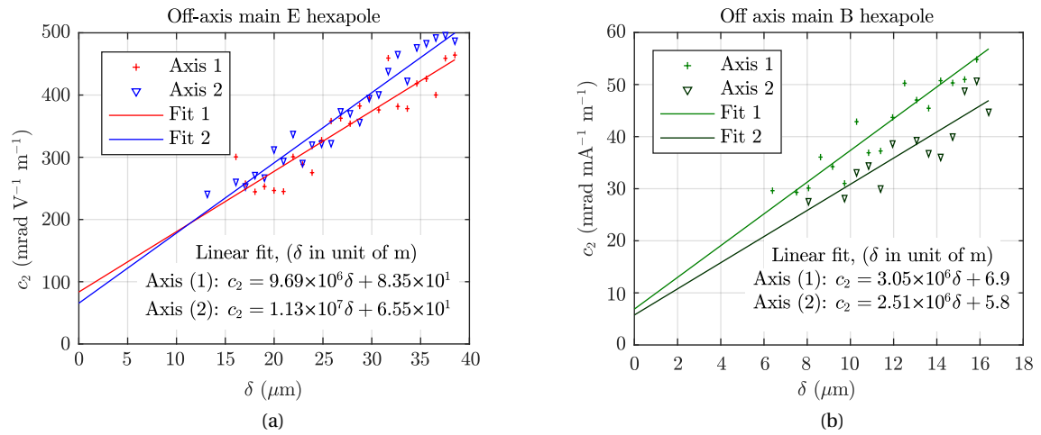
FIG. 14. (a) The obtained electric quadrupole magnitude c_2 as a function of the off-axis position in the bottom layer, for both axis and obtained for a 2 keV beam energy. From the slope, the hexapole field strength is approximated, c_{3,E} = 3.3 \times 10^5 \text{ mrad } V^{-1} m^{-2} . (b) The obtained magnetic quadrupole magnitude, as a function of the estimated average off-axis position in the middle layer magnetic field. From the slope, c_{3,B} = 9.27 \times 10^5 \text{ mrad } mA^{-1} m^{-2} is obtained.
