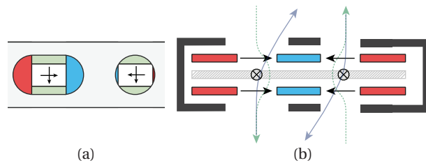
FIG. 5. Schematic representation of the electrodes and field orientation inside the beam separator for two parallel axes. (a) Top view showing the entrance apertures (grey) and inside electrodes. (b) Direction of the fields inside the device, with respect to the various electrodes. The field in the top and bottom layer always points in opposite direction for both axes. The central field is shared across both axes and thus performs an axis-independent action on the beam. Resulting beam trajectories for electrode excitations that satisfy the Wien condition are shown. The perpendicular cross section is unchanged from the single-axis design and not shown here again.
