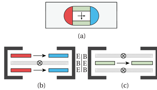
FIG. 3. Schematic representation of the electrodes and field orientation inside the beam separator. (a) Top view, with the elongated entrance slit (grey), primary electric (red and blue) and magnetic (green) poles visible. (b) Horizontal cross section view of the beam separator, with the in-plane electric field and out-of-plane magnetic field arrows. (c) Vertical cross section view, perpendicular to the view of (b), showing the direction of the generated fields. The signs of the fields are all interchangeable.
