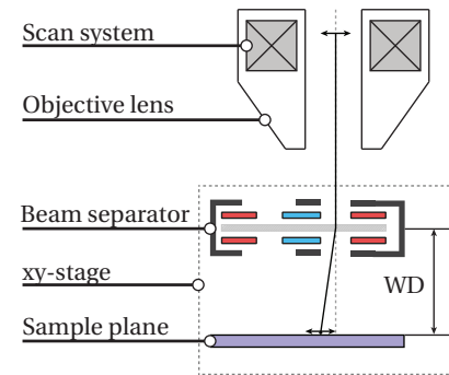
FIG. 10. Schematic of the experimental setup. The beam separator and specimen are placed together on an xy -translation stage inside the specimen chamber of the microscope. The scan system of the microscope provides the scanning and detector logic, and the beam is focused onto the specimen by the normal-mode objective lens of the microscope.
