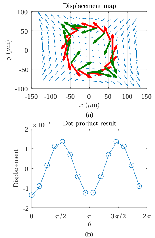
FIG. 11. Outline of the detection method. (a) The displacement map data is interpolated onto a regular spaced grid and the displacement map vectors are shown (blue arrows). The dot product is calculated for the analysis circle tangent vectors \vec{\kappa} (red arrow) and interpolated displacement vectors \vec{v} (green arrows). (b) Result of the dot product calculation for the displacement map shown, a sparse data set shown for clarity.
