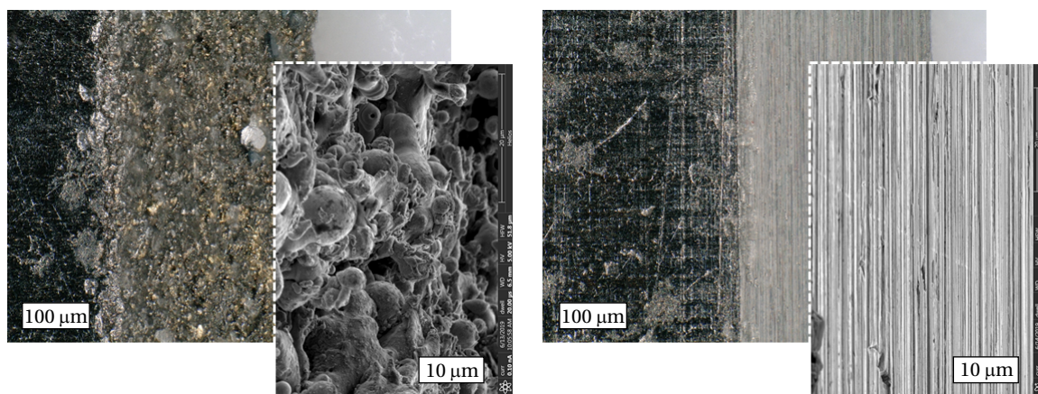
FIG. 7. Optical and SEM inspection photo- and micrograph (tilted) of a spark eroded electrode pole before (left) and after (right) polishing with a fine grain abrasive paper. Notice the yellowish colored sediment in the photograph of the unpolished electrode, which suggests that the spark wire deposits material onto the electrode. No traces of this deposited material were found after surface treatment.
