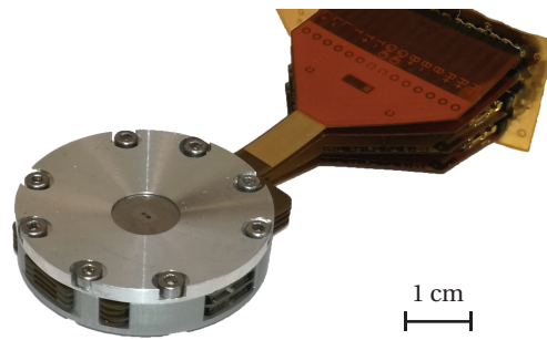
FIG. 9. Photograph of the assembled EBE separator that was used during the experiments. The outer diameter of the holder measures 38 mm and the total thickness of the device (including the cover) measures 9.4 mm.
