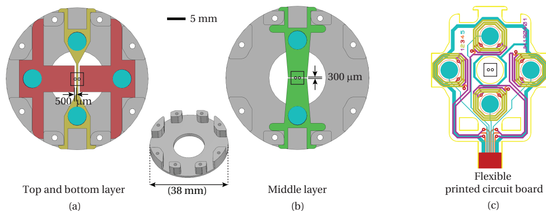
FIG. 8. Mechanical outline of the device enclosure (inset for perspective view) and shape and orientation for (a) the top and bottom layer electrodes and (b) the central layer electrodes. All electrodes are manufactured by spark erosion from mu-metal. The alignment of the elements relies on the tangent surfaces and grips at the circumference of the device enclosure. Electrical contact and magnetic flux injection is achieved through (c) the flexible printed circuit boards (fPCBs). The turquoise islands provide electrical contact for the electrodes and these are surrounded by 12 turn coils (distributed over four layers, 3 turns per layer). The circles inside the black square indicate the position of both optical axes.
