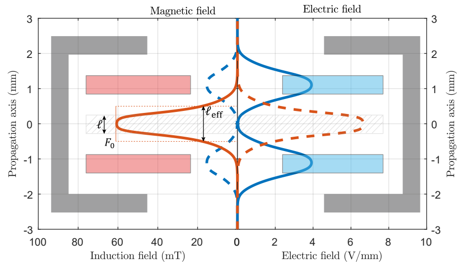
FIG. 4. Axial (left) magnetic induction, and (right) electric field strength components, for fields that provide a net force on the beam in the in-plane (solid) and out-of-plane (dashed) direction. An excitation current of 1 A, and potential of \pm 1 V were used for this calculation. The definitions for the electrode thickness ( \ell ) and effective field length ( \ell_{\text{eff}} ) are indicated for the middle layer.
