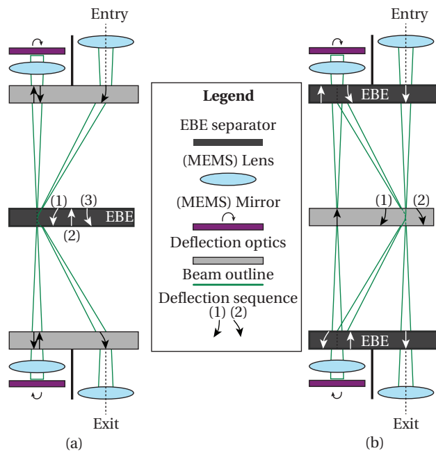
FIG. 1. MEMS based multi-axes electron optical setups, based on proposals for (a) miniaturized double electron mirror based aberration correction for scanning electron microscopy, and (b) mirror based beam patterning. The beam enters from the top on the right hand side axis, and propagates through the setup as indicated by the beam outline (green) and deflection sequence (numbered arrow). The use of MEMS electron optics enables small deflection angles (below 100 mrad), such as to limit deflection dispersion errors. The EBE separator units indicate optical planes that require a directional dependent deflection. Other deflection optics relies on electrostatic deflection fields only.
