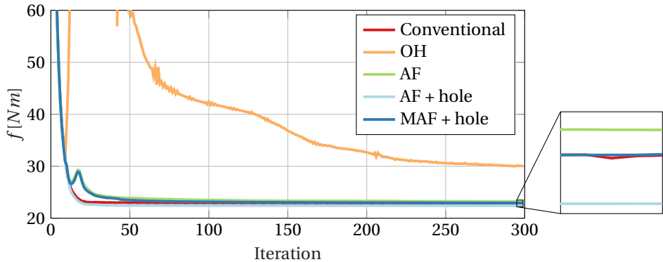
Figure 6.23: Convergence plots for the torsion box case for the conventional, overhang filter (OH), accessibility filter (AF), accessibility filter with force hole (AF + hole), and the modified accessibility filter with forced hole (MAF + hole).
