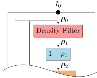
Figure 6.22: The modified accessibility filter with additional density filter as indicated by the red block. The remainder of the filter is similar to Figure 6.9.
