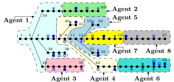
Fig. 2. The locations of non-dispatchable units (indicated by filled squares, ■), dispatchable generators (indicated by empty squares, □), and storage units (indicated by crosses, ×) in the PG&E 69-bus distribution network, which is partitioned into eight subsystems [29].
