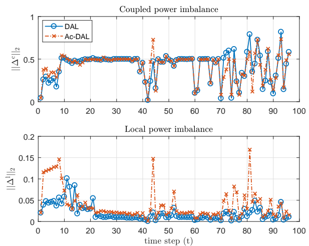
Fig. 5. Top plot shows the coupled power imbalance, \|\Delta^c\|_2 (see (17)). Bottom plot shows the local power imbalance, \|\Delta^l\|_2 (see (18)).
