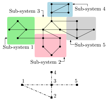
Fig. 1. An example of a small-scale energy network. Top figure shows graph \mathcal{G} where the nodes in \mathcal{N} are depicted as dots and the links in \mathcal{E} are depicted as solid lines. The graph \mathcal{G} is partitioned into five subsystems. Bottom figure shows graph \mathcal{G}^s where the subsystems in \mathcal{P} are depicted as filled squares and the links in \mathcal{E}^s are depicted as dash-dotted lines.
