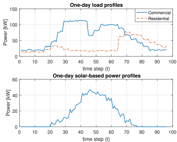
Fig. 3. One-day residential and commercial load profiles (top plot) and one-day solar-based power generation profile (bottom plot).
