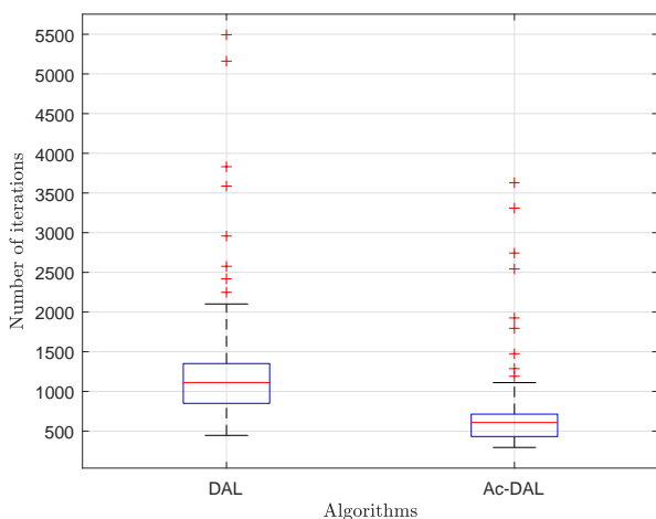
Fig. 4. The number of iterations performed by each algorithms. The blue boxes show the 25 th percentiles until the 75 th percentiles, the red lines show the median, and the + symbols indicate outliers.
