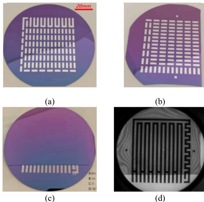
Fig. 7. Wafer-scale daisy chain pattern on the (a) bottom wafer, (b) trimmed top wafer and (c) bonded wafers. (d) Infrared light inspection of bonded wafers.
