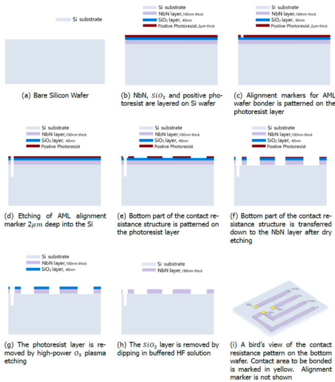
Fig. 5. Fabrication of contact resistance pattern on the bottom wafer.
