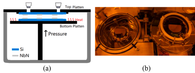
Fig. 4. (a). Illustration of the wafer bond (b) Top and bottom wafers loaded on the platens.
