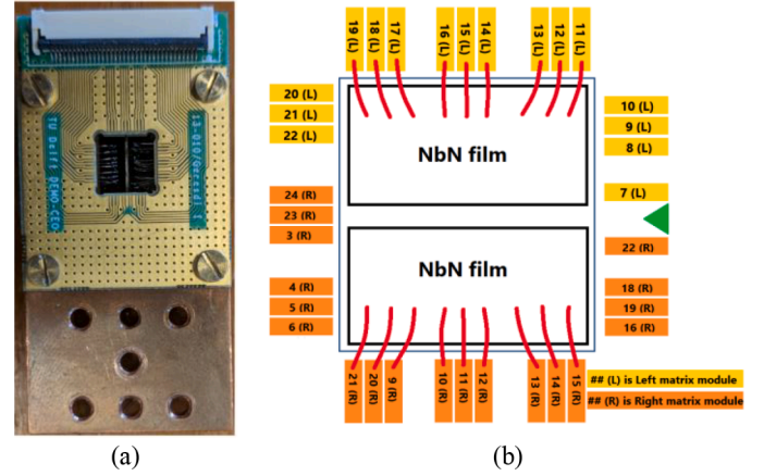
Fig. 1. (a) Sample of the NbN film glued to the PCB and (b) the wire-bonding scheme.
