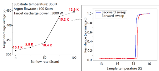
Fig. 9. Target discharge voltage as a function of N_2 flow rate with measured T_c attached. Subplot gives the normalized resistance versus computer-controlled sweeping temperature.
