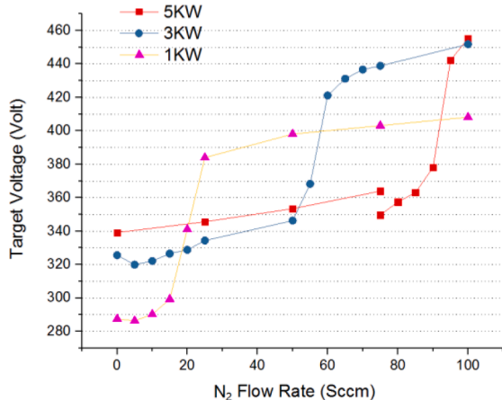
Fig. 8. Discharge voltage as a function of N_2 flow rate at target powers of 1 kW, 3 kW and 5 kW. The platen temperature is 350 °C and the Ar flow rate is 100 sccm.
