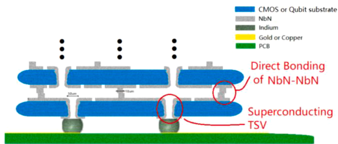
Fig. 12. Conceptual Schematic of a two(multi)-layer superconducting structure for 3-D qubit integration.
