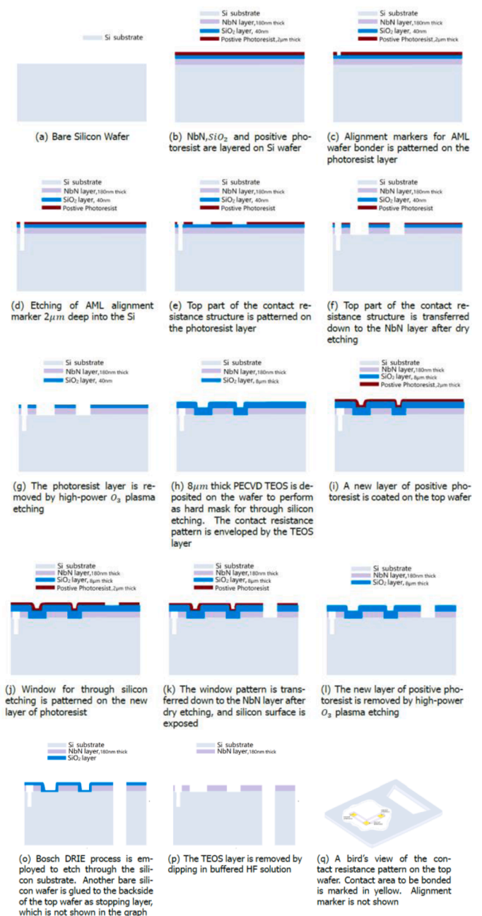
Fig. 6. Fabrication of contact resistance pattern on the top wafer.
