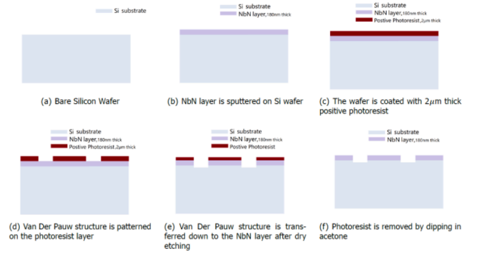
Fig. 2. Schematic of Van der Pauw structure fabrication process for measuring sheet resistance of NbN.
