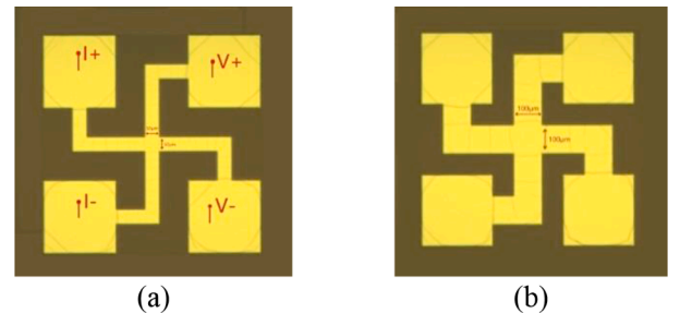
Fig. 3. Van Der Pauw structure of 180 nm-thick NbN film with central square size of (a) 50 \mu\text{m} \times 50 \mu\text{m} , (b) 100 \mu\text{m} \times 100 \mu\text{m} .
