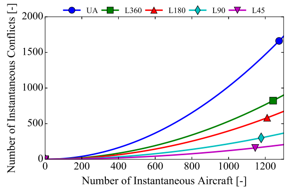
Fig. 11. Conflict rate for cruising aircraft (primary experiment). The curves represent the least-square fit of the simulation data to Eq. 3 for Unstructured Airspace (UA) and to Eq. 10 for the layered airspace concepts.
