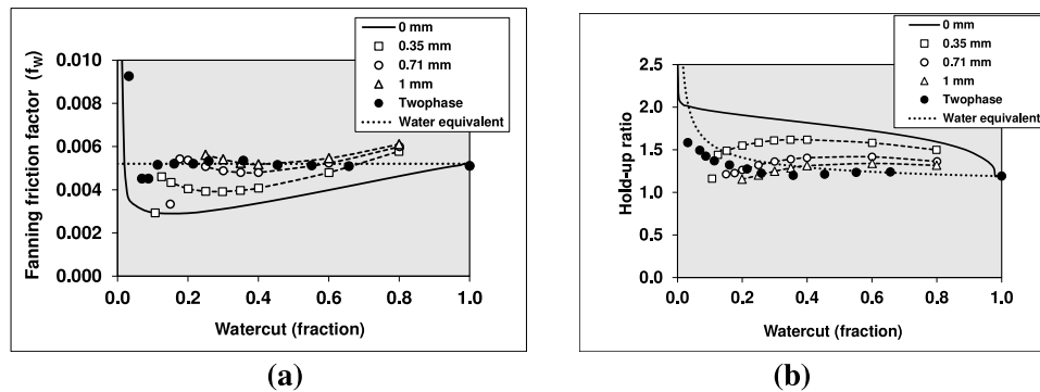
Figure 17. Single-phase simulations for the water annulus with sinusoidal wavy interface for the base case configuration with fixed total flow rate; dependence on watercut for (a) Fanning friction factor, (b) hold-up ratio.
