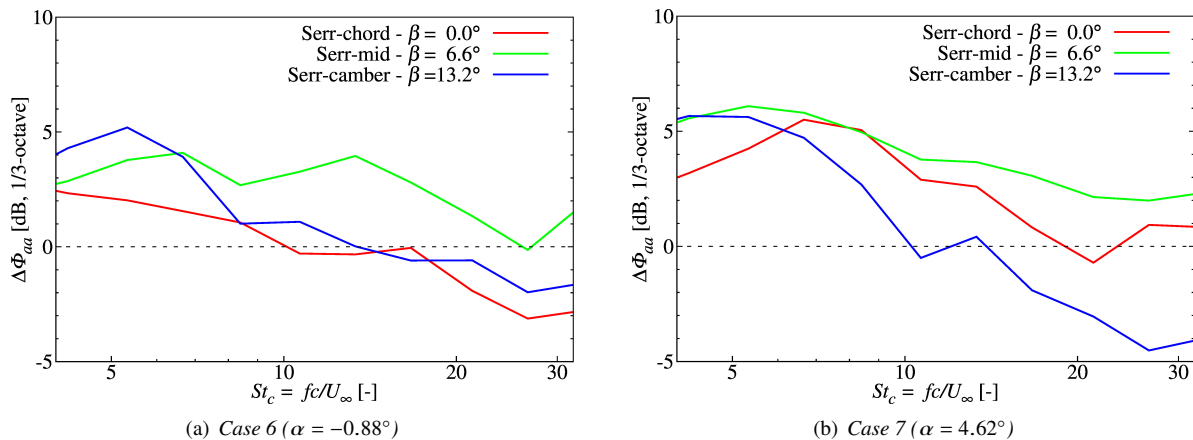
Fig. 12 Far-field noise reduction in 1/3-octave band \Delta\Phi_{aa} at (x = 0.19 \text{ m}, y = 1.62 \text{ m}, z = 0 \text{ m}) . A positive value of \Delta\Phi_{aa} has the meaning of noise reduction with respect to the straight trailing-edge.
