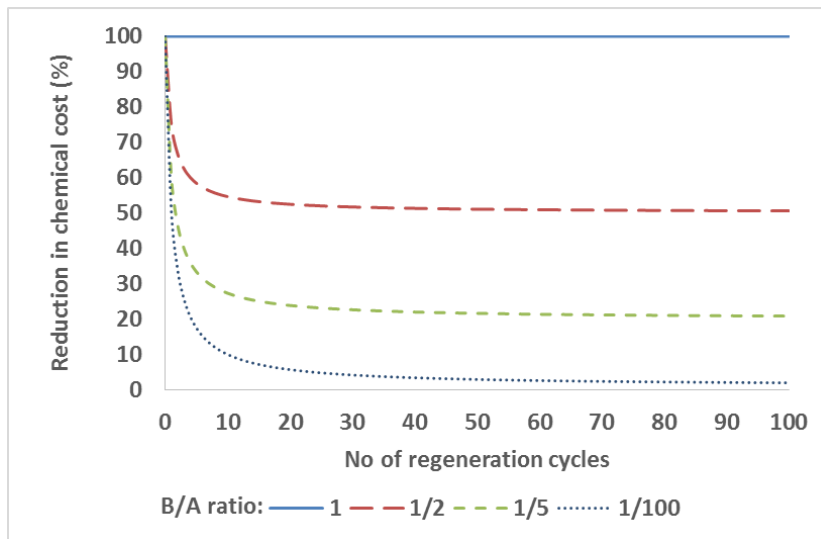
Figure 7-5: The decrease in chemical cost of adsorption as a function of the number of regeneration cycles. The legends show the ratio of the terms B/A , i.e. the cost per regeneration cycle as compared to the cost of the 1 st adsorption cycle.
