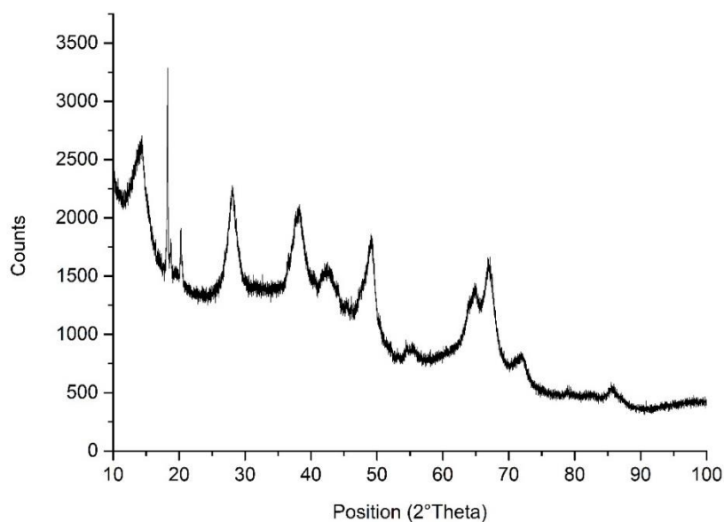
Figure S4-8: XRD spectrum of DD6. The peaks at position 18.2, 18.7, 20.3 correspond with aluminium oxide (Al 2.67 O 4 ), whereas the peak at 13.9 corresponds with aluminium oxide hydroxide (AlO(OH)). Peaks at positions 28.1, 32.6, 38, 42.8, 48.9, 54.8, 64.4, 67, 71.8, 85.6 correspond with both aluminium oxide and aluminium oxide hydroxide.
