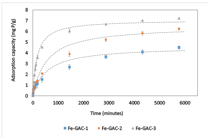
Figure S3-11: Adsorption kinetics of the Fe-GACs. Dashed lines represent the pseudo second order kinetic model fit. (Initial phosphate concentration = 20 mg P/L, Adsorbent concentration = 2 g/L, pH \approx 6.5)
