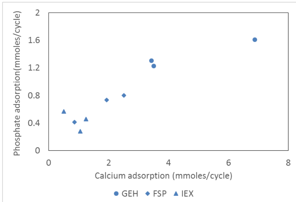
Figure 6-7: Correlation of Ca vs P adsorption (including all cycles for all adsorbents using acid-alkaline regeneration)
