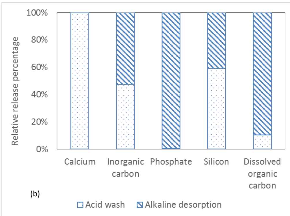
Figure S6-13: Relative release of different molecules in acid wash and alkaline desorption during acid-alkaline regeneration for (a) GEH and (b) IEX
