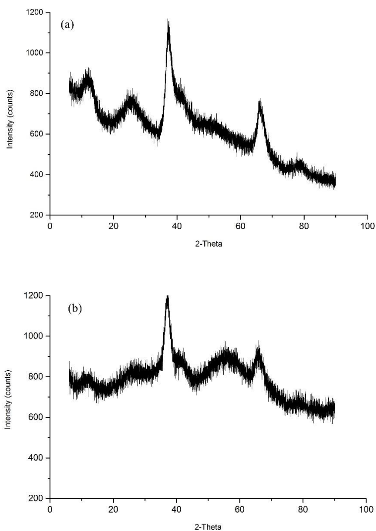
Figure S3-12: XRD spectra of (a) GAC-3 oxidized with KMnO_4 (b) Fe-GAC (GAC-3 with highest iron loading)
