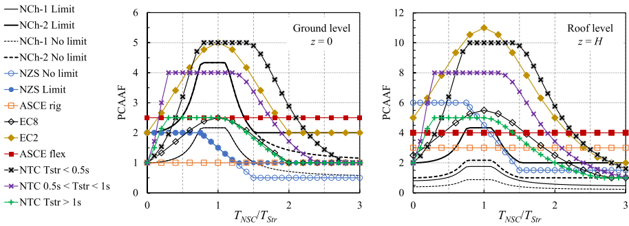
Fig. 4 Comparison of PCAAF for ground and roof levels. Note for NZS, T_{Str}=1 to enable comparisons with the prescriptions of the other codes
