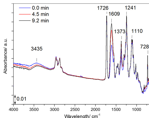
Fig. 5. Chemisorption kinetics of uncured polyester coat applied on native zinc oxide, collected using p-polarized IR-light.
