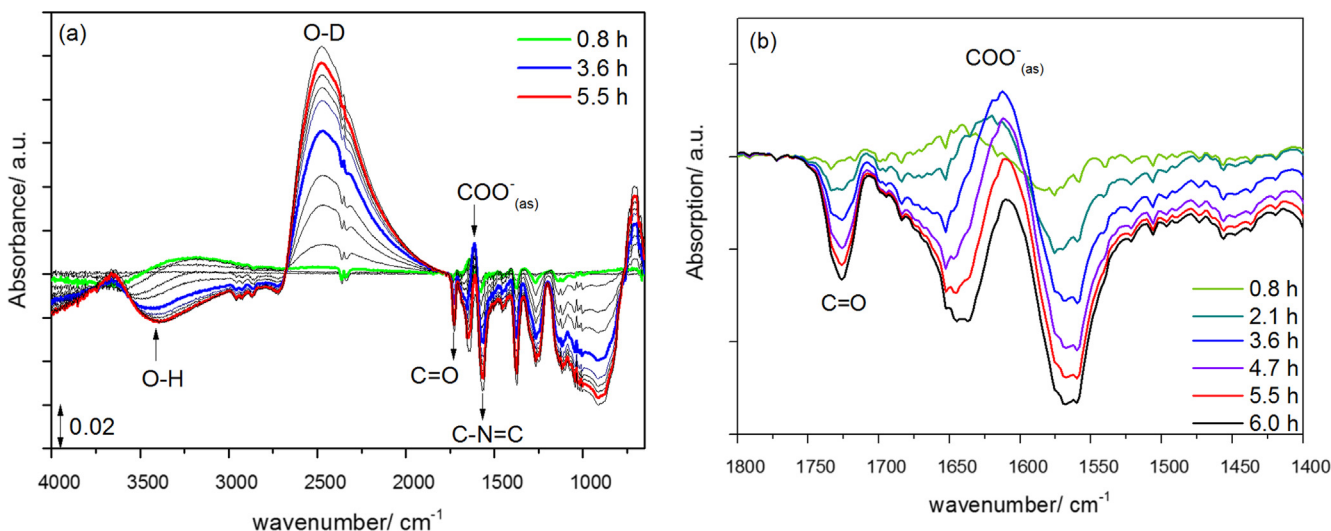
Fig. 10. ATR-FTIR spectra of D 2 O permeation through polyester coating applied on hexafluorozirconic acid treated zinc (a) full scale, (b) enlarged carboxylate region.
