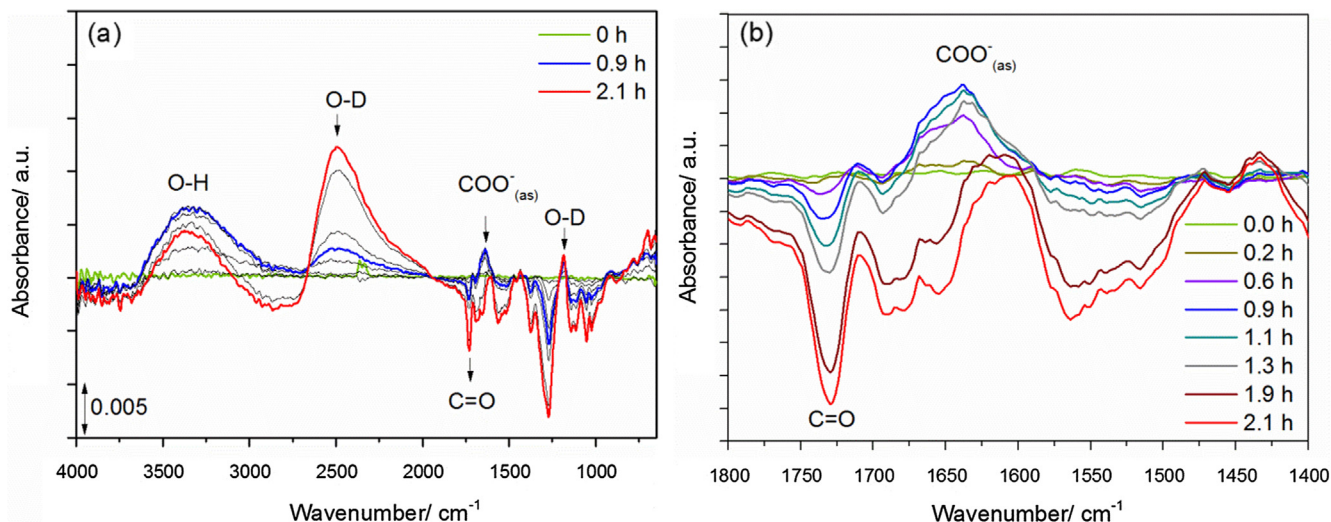
Fig. 8. ATR-FTIR spectra of D 2 O permeation through polyester coating applied on native zinc oxide (a) full scale, (b) enlarged carboxylate region.
