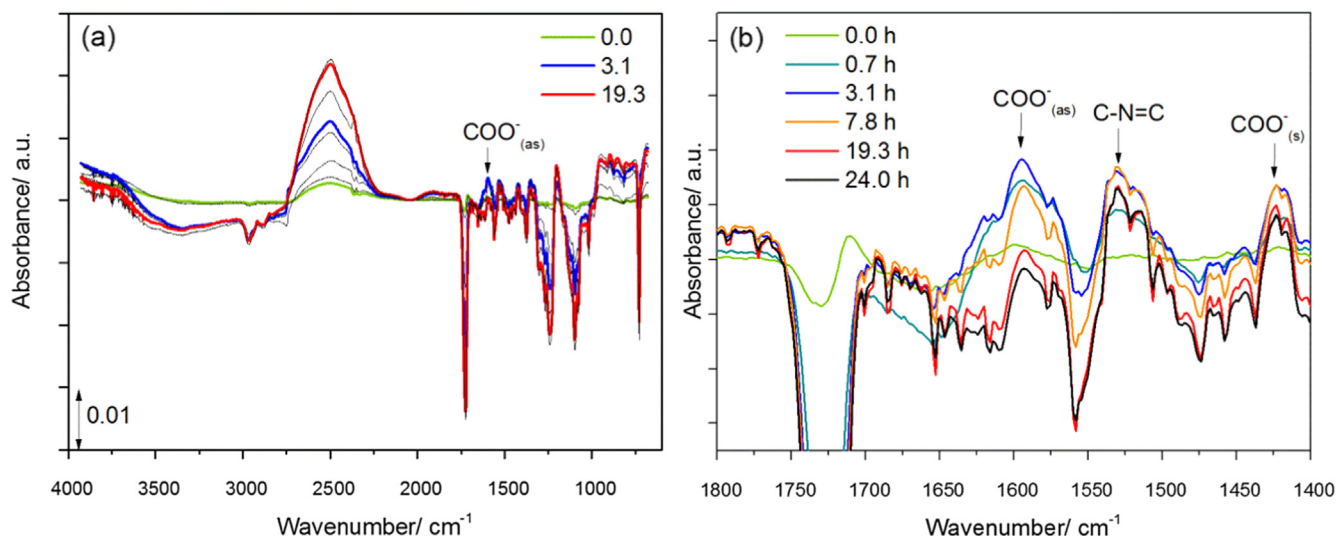
Fig. 12. ATR-FTIR spectra of D_2O permeation through polyester coating applied on hexafluorozirconic acid treated magnesium oxide (a) full scale, (b) enlarged carboxylate region.
