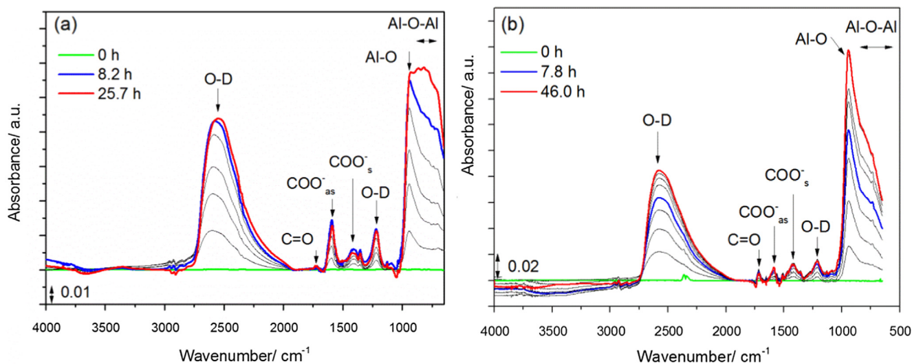
Fig. 13. ATR-FTIR spectra of D_2O permeation through polyester coating applied on (a) untreated and (b) zirconium-based treated aluminium.
