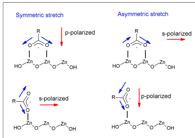
Fig. 7. Transition dipole moments of asymmetric and symmetric carboxylate stretch vibrations in different coordination modes.
