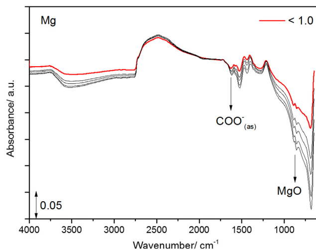
Fig. 11. ATR-FTIR spectra of D 2 O permeation through polyester coating applied on native magnesium oxide.
