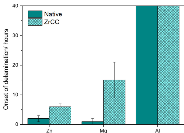
Fig. 14. Onset of delamination based on infrared peak area of asymmetric carboxylate stretching vibration followed in-situ during exposure to D_2O .
