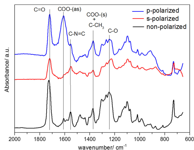
Fig. 6. ATR-FTIR spectra of cured polyester coating applied on zinc coated germanium internal reflection element, collected using p-polarized, s-polarized and non-polarized IR-light with an incident angle of 80°.
