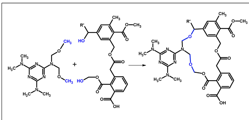
Fig. 3. Crosslinking reaction between CH 3 groups of the melamine-based crosslinker and OH-groups of the polyester resin.
