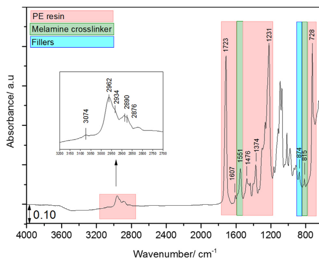
Fig. 1. ATR-FTIR spectrum of cured polyester coating applied on germanium internal reflection element, collected using non-polarized IR-light at an incident angle of 80°.
