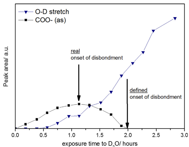
Fig. 9. Peak area dynamics of polyester coated zinc as a function of exposure time to D 2 O.
