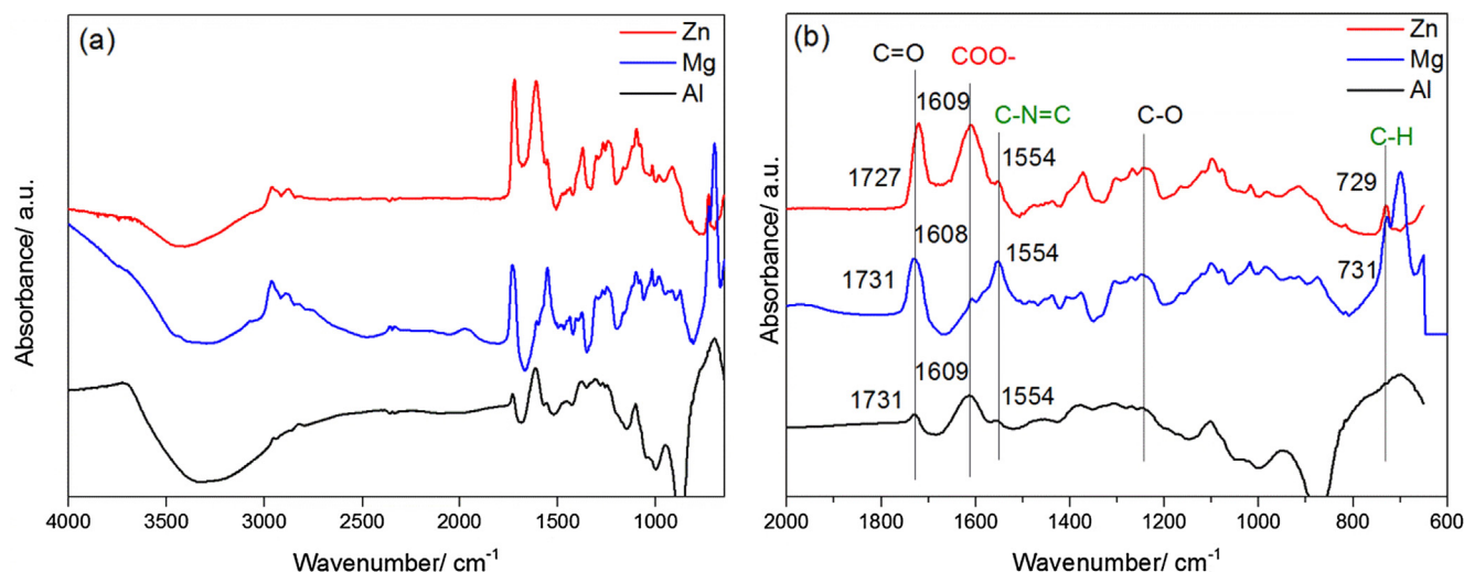
Fig. 2. ATR-FTIR spectra of cured polyester coating applied on native zinc, magnesium and aluminium oxide, collected using p-polarized IR-light with an incident angle of 80^\circ (a) full scale, (b) head group region.
