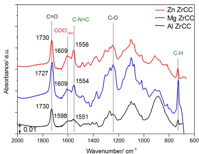
Fig. 4. ATR-FTIR spectra of cured polyester coating applied on hexafluorozirconic acid treated (ZrCC) zinc, magnesium and aluminium, collected using p-polarized IR-light with an incident angle of 80°.
