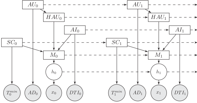
Fig. 4. The graph representation of the DBN from [1]. Rectangular nodes are discrete, round nodes are continuous. Gray nodes indicate measured values.
