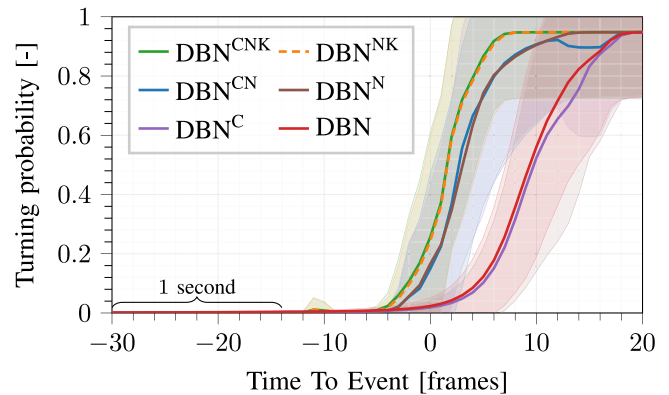
Fig. 7. The mean (lines) and one-sigma standard deviation (shaded area) of the turning probability for the normal turning tracks. The turning probability is most in line with the annotated moment of turning when all parameters are optimized ( DBN^{CNK} , green line, and DBN^{NK} , dashed orange line).
