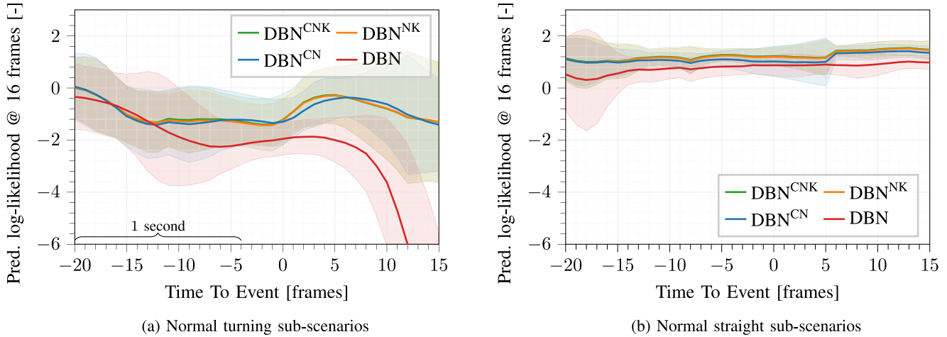
Fig. 6. One second ahead prediction log-likelihood mean (thick line) and one-sigma standard deviation (shaded area) of DBNs over time. In the turning sub-scenarios (Fig. 6(a)), the performance of the DBN with no additional parameter optimization (DBN, red line) deteriorates after TTE = 5 . The optimized DBNs do not see this deterioration. In the straight scenario (Fig. 6(b)), optimization improves performance.
