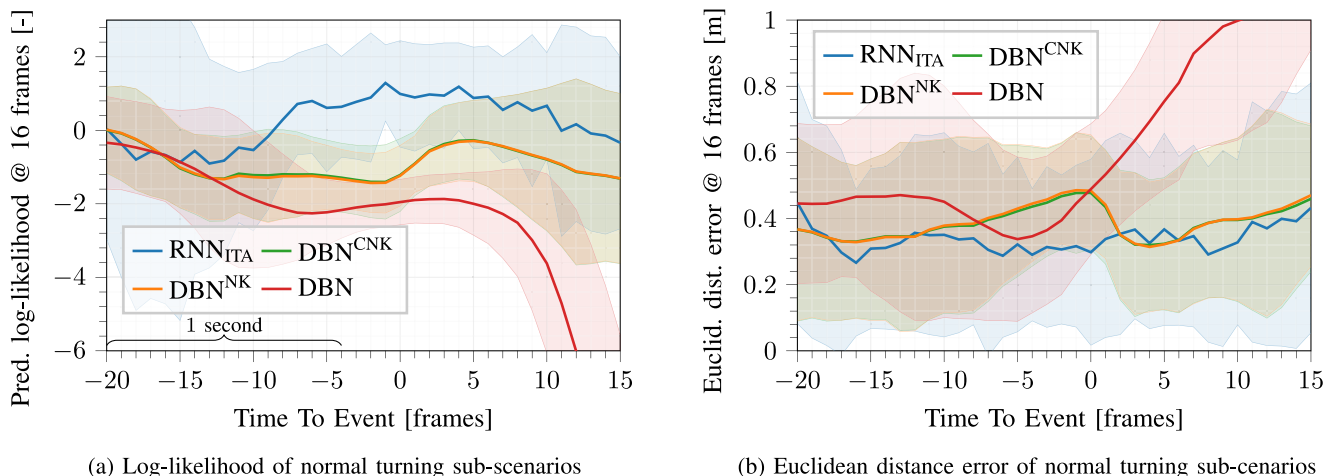
Fig. 8. The mean (lines) and one-sigma standard deviation (shaded area) of the one second ahead prediction log-likelihood (Fig. 8(a)) and Euclidean distance error (Fig. 8(b)) for the normal turning sub-scenarios.
