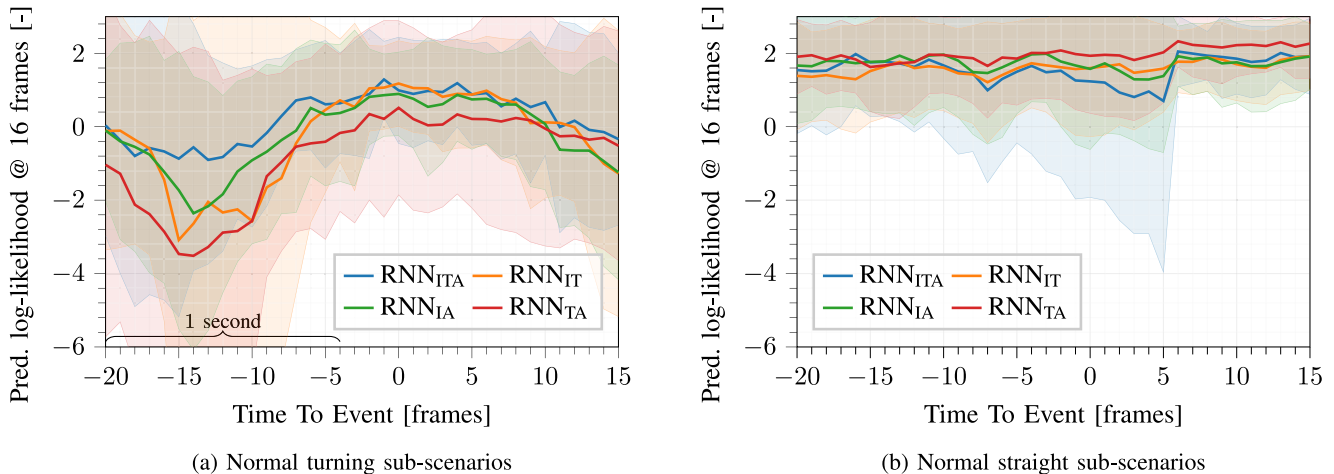
Fig. 5. One second ahead prediction log-likelihood mean (thick line) and one-sigma standard deviation (shaded area) of RNNs over time. When turning (Fig. 5(a)), the RNN with all three context cues (RNN ITA , blue line) performs the best.
