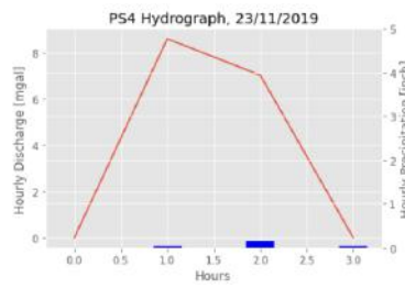
Figure 5.17: Hydrograph for peak 5 for DPS 4
