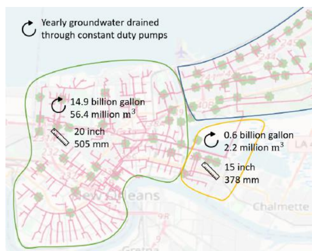
Figure 5.24: Yearly groundwater flow through constant duty pumps
