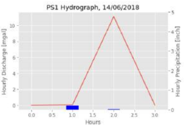
Figure 5.10: Hydrograph for peak 4 for DPS 1
