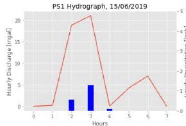
Figure 5.11: Hydrograph for peak 5 for DPS 1
