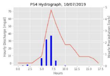
Figure 5.16: Hydrograph for peak 4 for DPS 4
