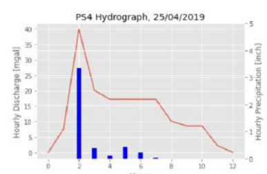
Figure 5.15: Hydrograph for peak 3 for DPS 4
