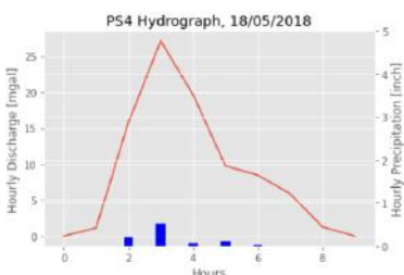
Figure 5.13: Hydrograph for peak 1 for DPS 4
