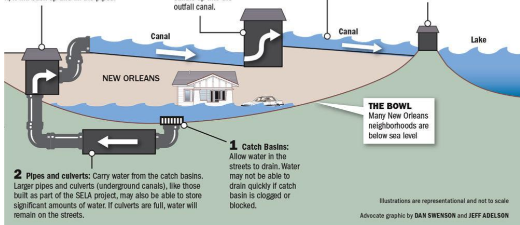
Figure 5.1: Explanation of storm water drainage system [Adelson, 2017]
