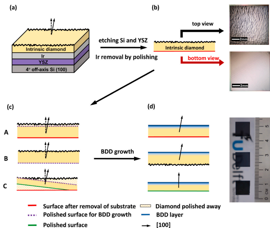
Fig. 1. Schematic displaying the fabrication of the three heteroepitaxial SC-BDD electrodes. (a) The layered stack was subjected to etching to remove YSZ and Si(100) and then to polishing to remove the Ir layer, which resulted in (b) free-standing, heteroepitaxially grown intrinsic diamond with 4° off-axis (100) plane, whose top and bottom views were visualized by a digital microscope. (c) The intrinsic diamond was further processed: For samples A and B, 4° off-axis was preserved, and the top (growth) side of sample A was polished (the back side of both samples was already polished due to Ir layer removal), while sample C was polished on both sides to eliminate the off-axis angle. (d) BDD layers were grown either on the polished top side (samples A and C) or the back side (sample B; flipped by 180° prior to BDD growth step) of the heteroepitaxial diamond quasi-substrate. Prepared (100)-faceted SC-BDD electrodes (1 cm 2 ) are shown in the picture (ruler with cm-scale). (A colour version of this figure can be viewed online.)
