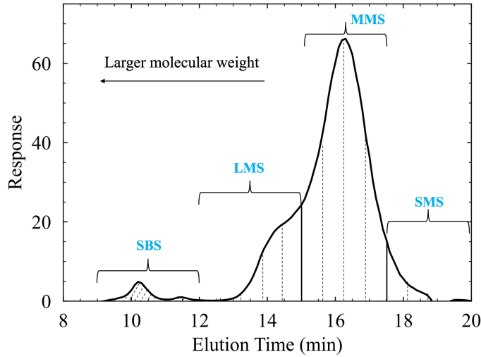
Figure 4.4 GPC chromatogram of bitumen.
