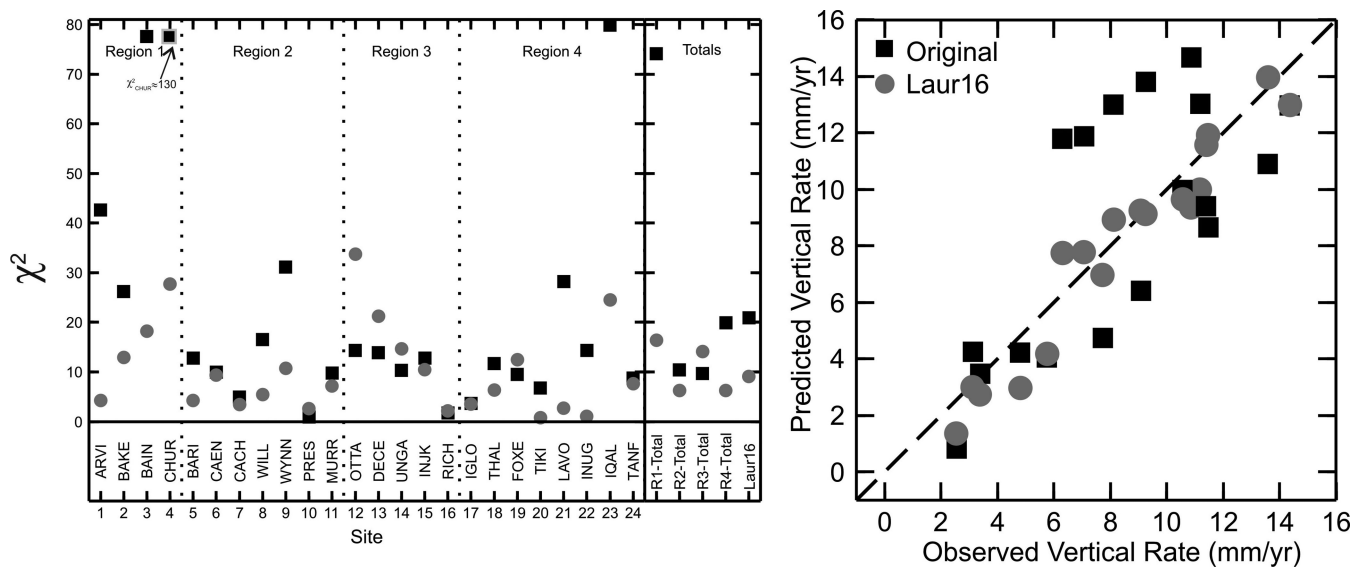
Figure 14. Summary of the fit of the original ice sheet reconstruction (black squares) and the best-fitting ice sheet reconstruction (grey circles, Laur16) to all RSL and GPS measurements in Regions 1–4. The left panel shows the \chi^2 misfit values for each of the individual RSL sites, as well as the cumulative \chi^2 misfit values for each region (R1-Total, R2-Total, R3-Total and R4-Total) and all regions (Laur16). The overall \chi^2 misfit value on the RSL data decreases from 21.0 for the starting model to 9.1 for the best-fitting Laur16 model. Note that the \chi^2 misfit value at Churchill plots off the vertical scale (at approximately 130). The right panel shows the predicted versus observed vertical uplift rates for the original model (black squares) and the Laur16 model (grey circles) for all 18 GPS sites. The overall MSE misfit value on the GPS data decreases from 9.0 \text{ mm}^2 \text{ yr}^{-2} for the starting model to 1.0 \text{ mm}^2 \text{ yr}^{-2} for Laur16.
