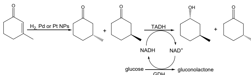
Scheme 1. Reduction of the \text{C}=\text{C} double bond with Pd or Pt NPs in tandem with the asymmetric reduction of the keto group by TADH. The reaction was performed under 10 bar \text{H}_2 at 30 °C in phosphate buffered solution, using glucose dehydrogenase (GDH) and glucose as the nicotinamide cofactor ( \text{NADH} ) regeneration system.
