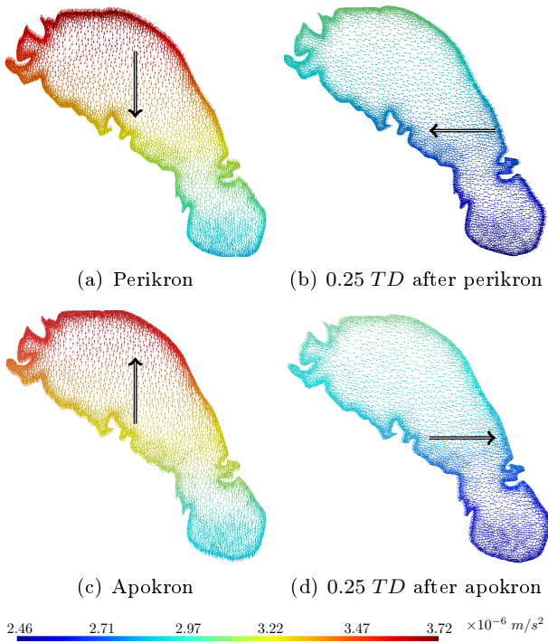
Fig. 4 Instantaneous maps of the acceleration caused by Saturn in Ontario Lacus at four different times (perikron, 0.25 TD after perikron, apokron and 0.25 TD after apokron)(the black arrows represent the mean direction). It rotates clockwise with an exact period of 1 TD and it is maximum in the northern part of the lake
