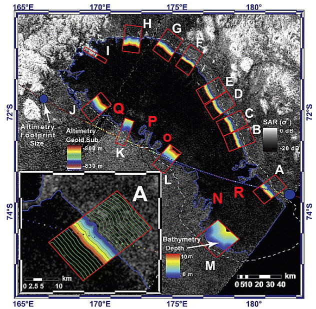
Fig. 1 Map of Ontario Lacus. Letters from A to M show the study areas of Hayes et al (2010) which derived a nearshore bathymetry in these regions. The red letters, from N to R, are used in this article to refer to particular areas. Credit: Radar Science Team, NASA/JPL/Caltech
