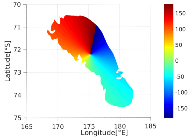
(b) Tidal phase of the main component (in degrees)
