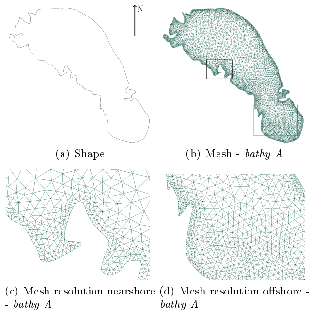
Fig. 3 Discretization of Ontario Lacus using mesh-generation package GMSH: the coastline (Panel (a)) and the mesh used for bathy A (Panel (b)). Panel (c) shows the higher spatial resolution nearshore. Panel (d) shows the refinement in shallow regions in bathy A
