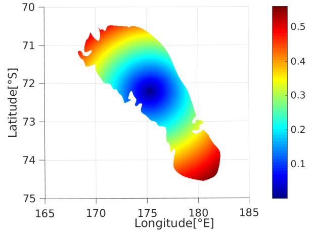
(a) Tidal range of the main component (in meters)
