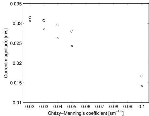
Fig. 14 Evolution of maximum current speed with respect to the Manning's friction coefficient at two different times: perikron (circle) and apokron (cross). As expected, the flow decreases as the bottom friction increases
