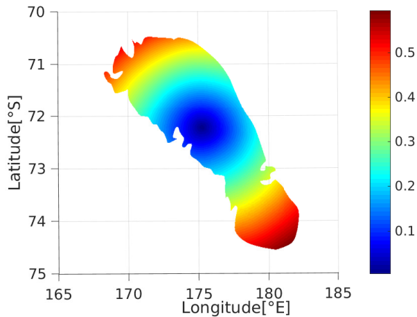
Fig. 15 Lake surface elevation range in Ontario Lacus with a southerly wind of 1 \text{ m s}^{-1} blowing during 1 \text{ TD} . It is higher in the south (due to the higher contribution of the constant term): the maximum lake surface elevation range is 0.593 \text{ m}
