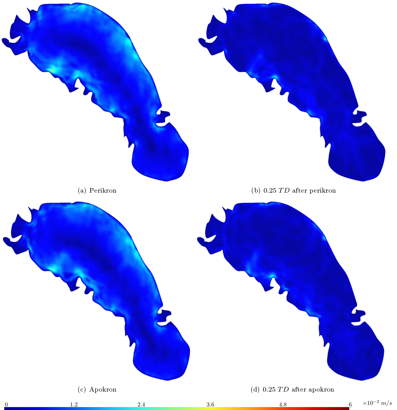
Fig. 7 Tidal current magnitude (in \text{ms}^{-1} ) in Ontario Lacus at (a) Perikron, (b) 0.25 TD after Perikron, (c) Apokron and (d) 0.25 TD after Apokron with bathy C implemented. The current magnitude is maximum nearshore, at areas P or Q (see Fig. 1), depending on the time, and decreases with the distance to the shore. Globally, the speed is higher in perikron and apokron than 0.25 TD after perikron and apokron
