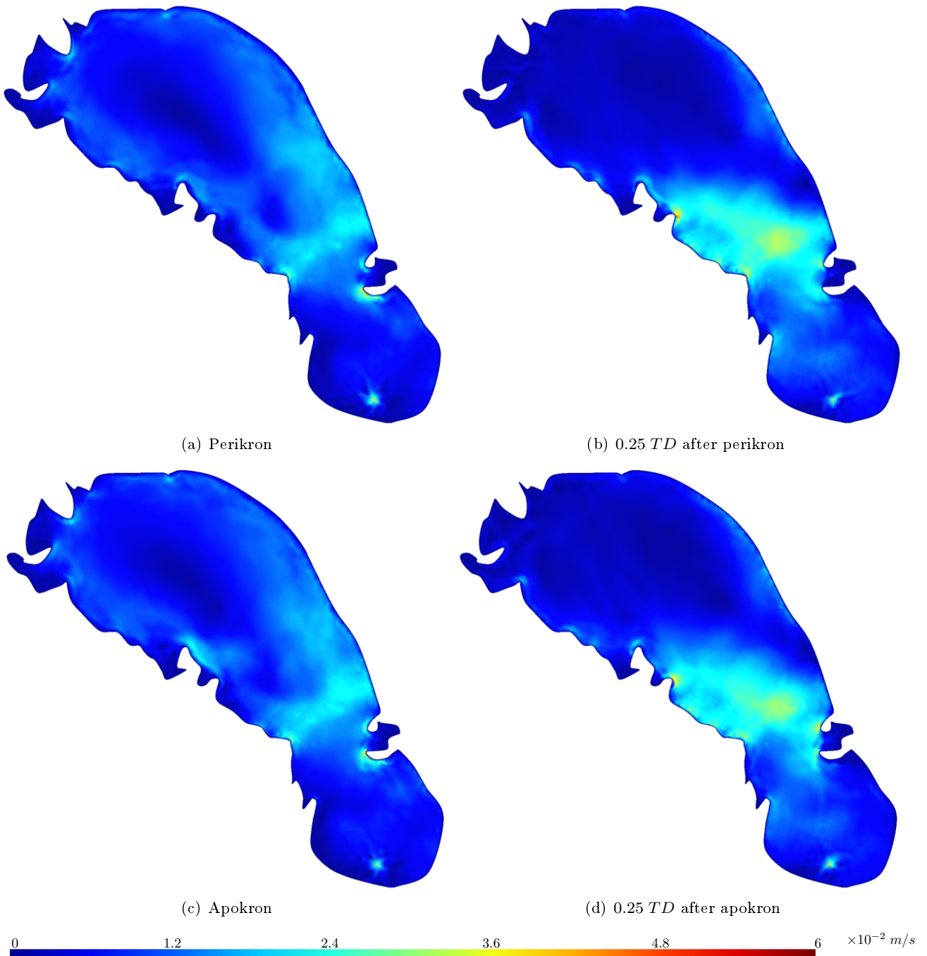
Fig. 9 Tidal current magnitude (in \text{ms}^{-1} ) in Ontario Lacus with bathy A implemented at (a) Perikron, (b) 0.25 TD after Perikron, (c) Apokron and (d) 0.25 TD after Apokron. The current magnitude is maximum nearshore, at area 0 (see Fig. 1) and decreases with the distance to the shore except near area N and R where a wide offshore unidirectional high speed area is predicted
