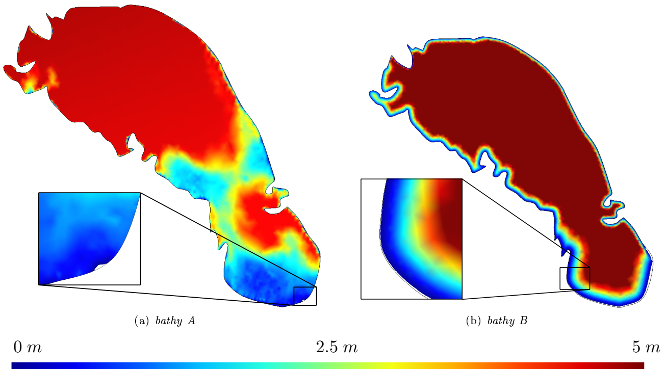
Fig. 13 Map of the total liquid depth (bathymetry + surface elevation) respectively with bathy A (Panel (a)) and bathy B (Panel (b)) implemented. The depth is cropped at 5 m in order to highlight the dry areas generated by tidal motion and the areas where there is not much liquid remaining. Most of the dry areas are located in the south while shallow areas can also be found offshore and on the eastern shore and on the north-western shore for bathy A . With bathy B implemented, there are more dry areas and they are larger
