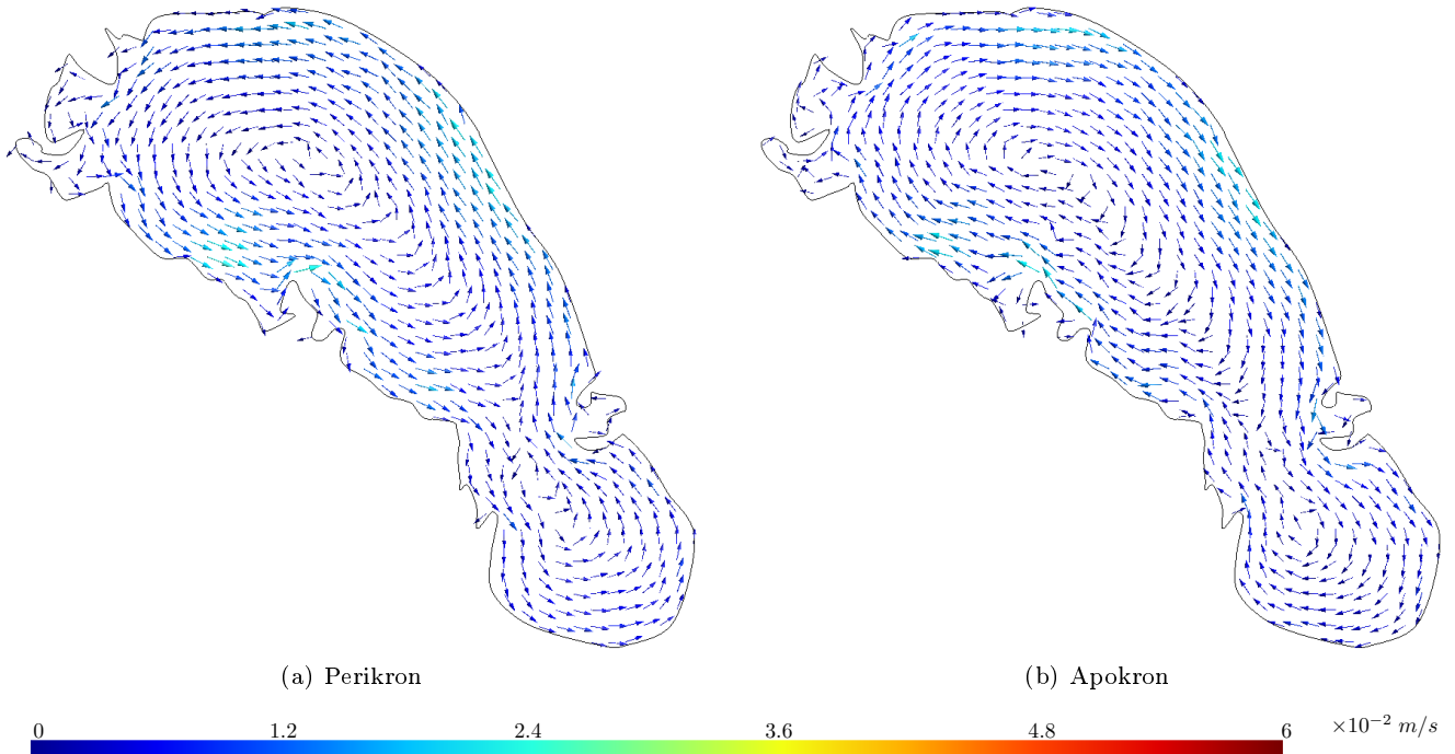
Fig. 8 Tidal current orientation in Ontario Lacus at (a) Perikron, and (b) Apokron with bathy C implemented (the flow is interpolated on a structured grid in order to increase the quality of the figure). This pattern rotates anticlockwise at perikron and clockwise at apokron
